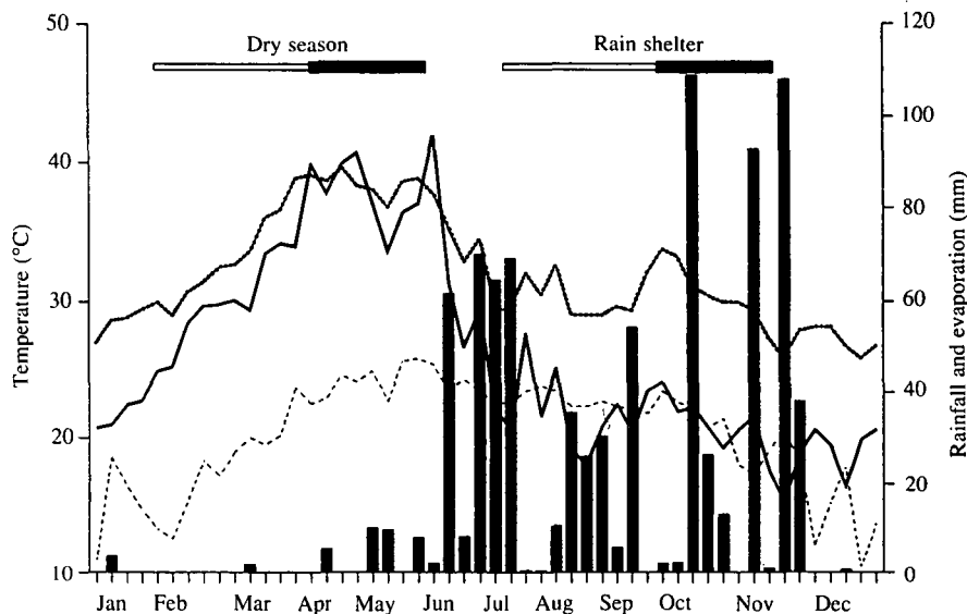
Fig. 1. Total weekly rainfall (bars), evaporation (—) and mean weekly minimum (-----) and maximum (-----) temperatures at Patancheru, India, during 1987. The cropping seasons in the irrigated dry season and rain-sheltered rainy season experiments are indicated by the horizontal bar; the drought-stress periods are indicated by the solid portion of the bar.
