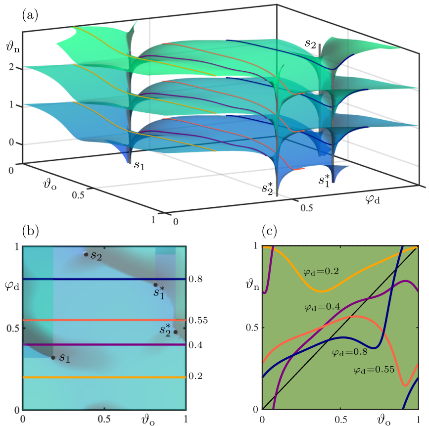
FIGURE 9. Panel (a) shows three copies of the phase-resetting surface \text{graph}(\mathcal{P}_A) of system (2.1) in (\vartheta_o, \varphi_d, \vartheta_n) -space for \vartheta_n \in [-0.5, 2.5] with A = 0.6 , featuring four singularities s_1 , s_2 , s_1^* and s_2^* (grey vertical lines); also shown are the four PTCs for \varphi_d = 0.2 (orange), \varphi_d = 0.4 (purple), \varphi_d = 0.55 (red) and \varphi_d = 0.8 (blue). Panel (b) is a projection of panel (a) onto the (\vartheta_o, \varphi_d) -plane and panel (c) shows the four PTCs on the fundamental square (green shading) of the (\vartheta_o, \vartheta_n) -plane.
