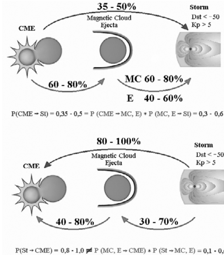
Figure 1. Schematic view of correlations between CME, MC/ejecta and magnetic storms for direct (top panel) and back (bottom panel) tracings. Relations of probabilities for 1- and 2-step tracings are shown below each panels
