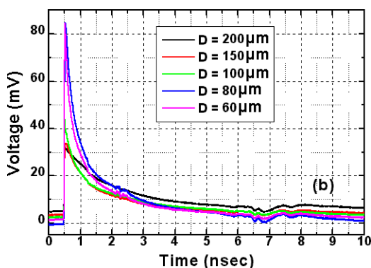
Figure 8b. The area dependence of pulse responses measured at 357 nm. (b) ITO-Schottky RCE-PD
