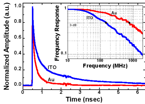
Figure 11. Normalized pulse responses of 30 \mu\text{m} -diameter Au and ITO-Schottky RCE-PDs with 77 ps and 154 ps FWHM respectively. Inset shows the corresponding FFT curves.
