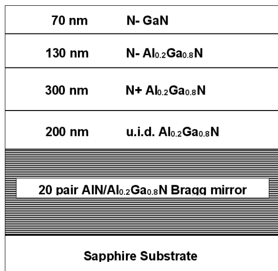
Figure 1. Epitaxial layer structure of the designed AlGa N RCE Schottky PD.
