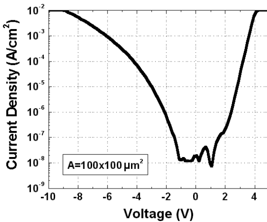
Figure 4. Measured dark current density of a 100 \times 100 \mu\text{m}^2 ITO-Schottky PD.
