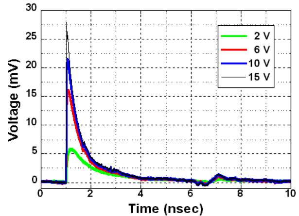
Figure 7. Pulse response of a 150 \times 150 \mu\text{m}^2 Au-Schottky RCE-PD as a function of reverse bias.
