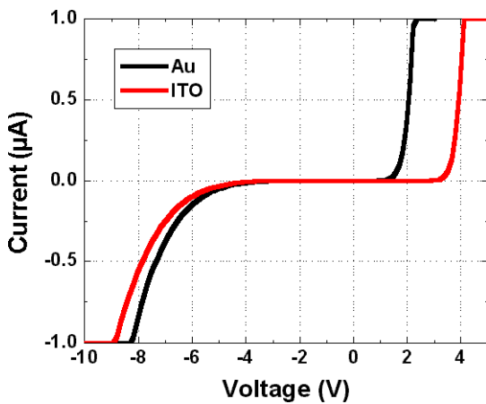
Figure 3. Typical I-V characteristics of 100 \times 100 \mu\text{m}^2 Au and ITO-Schottky RCE-PDs.
