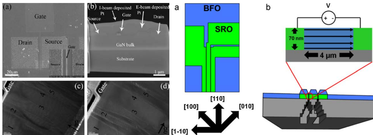
Figure 1. (a) SEM image of a typical AlGaN/GaN HEMT in the pristine (unbiased) state, (b) Crosssection view of the lift-out indicates the features of the device as well as the Pt protective layers. (c) and (d) represent weak-beam dark-field TEM images of drain-gate region at two different diffraction conditions of g \frac{1}{4} \frac{1}{2} 0002 and g \frac{1}{4} \frac{1}{2} 1120 , respectively. Scale bars are 200 nm and the threading dislocations are labeled as 1–5, from [1]
