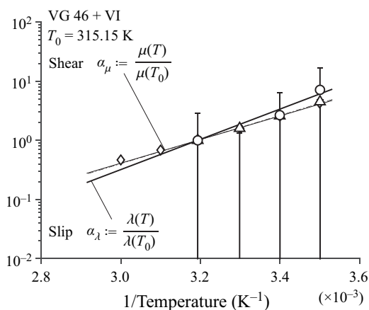
Figure 22. Arrhenius plot for bulk shear obtained by the SLT, a reference viscometer and wall slip for the ISO VG 46 + VI. The solid lines show the results obtained by the SLT, whereas the dashed line and diamond markers represent the results by the viscometer. The activation energy for bulk shear obtained by the SLT is E_\mu = 38.2 \text{ kJ mol}^{-1} and for wall slip E_\lambda = 48.9 \text{ kJ mol}^{-1} .
