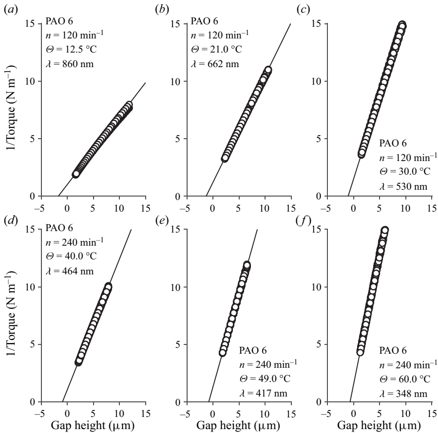
Figure 9. Slip length measurements for a synthetic hydrocarbon alpha-olefin (PAO 6). The temperature was varied in a range of 12.5 \text{ }^\circ\text{C} \leq \Theta \leq 60.0 \text{ }^\circ\text{C} . The measurement uncertainty of gap height and torque are so small that the uncertainty intervals are hidden behind the markers. Nevertheless, the existing uncertainties are taken into account in the uncertainty propagation according to Appendix B to determine the measurement uncertainty of the slip length.
