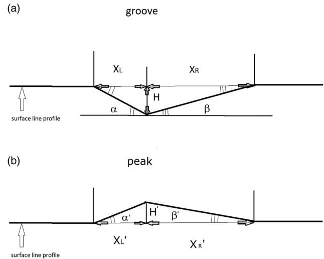
Fig. 2. Schematic of AFM line profile measurements showing the direct measurements of the depth H for the groove (a) and the height H' for the peak (b). The half-width distance to the left, X_L , and to the right, X_R , from the min/max point of the grooves and peaks are shown. The angles, \alpha and \beta , calculated from the vertical and horizontal distance measurements are also shown.
