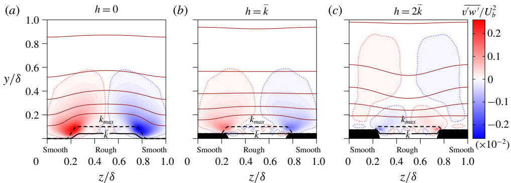
FIGURE 6. Reynolds stress \overline{v'w'} at different elevations of the smooth stripes h . Brown solid lines mark the isolines for the streamwise mean velocity distribution with isolevels corresponding to figure 4.
