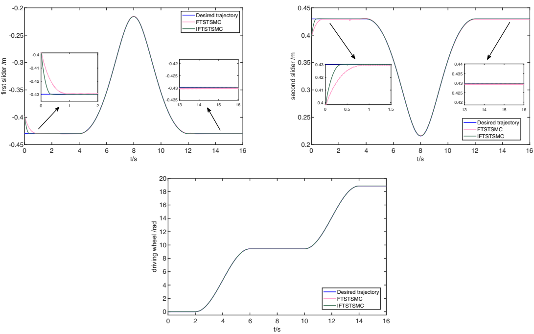
Figure 8. Tracking trajectory curves of sliders and driving wheel.
