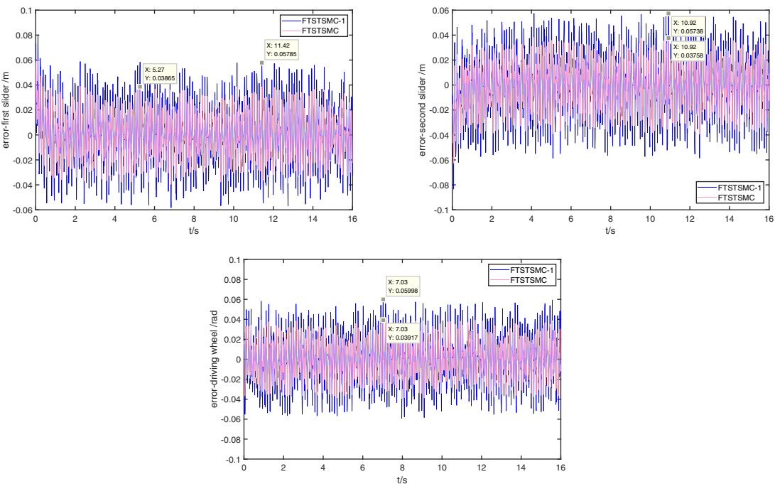
Figure 16. Experimental results of tracking errors for FTSTSCM-1 and FTSTSMC.
