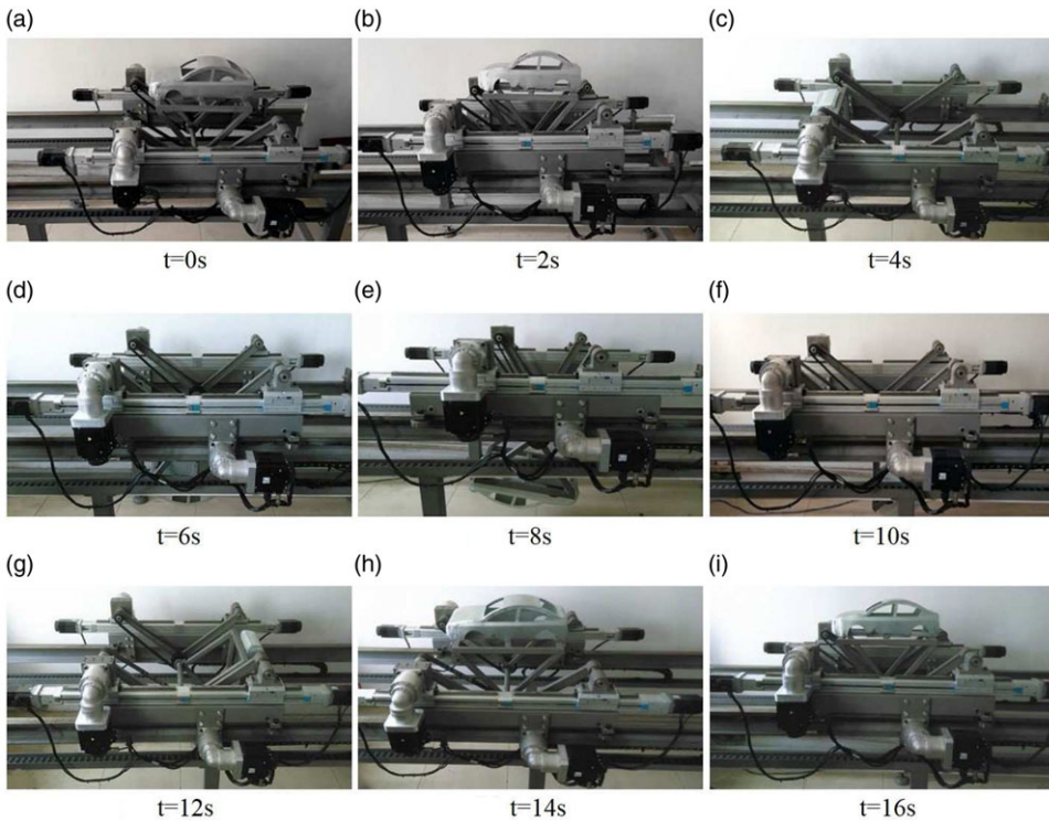
The pose of the hybrid mechanism used for automobile electro-coating conveying at different moments in the operation.
