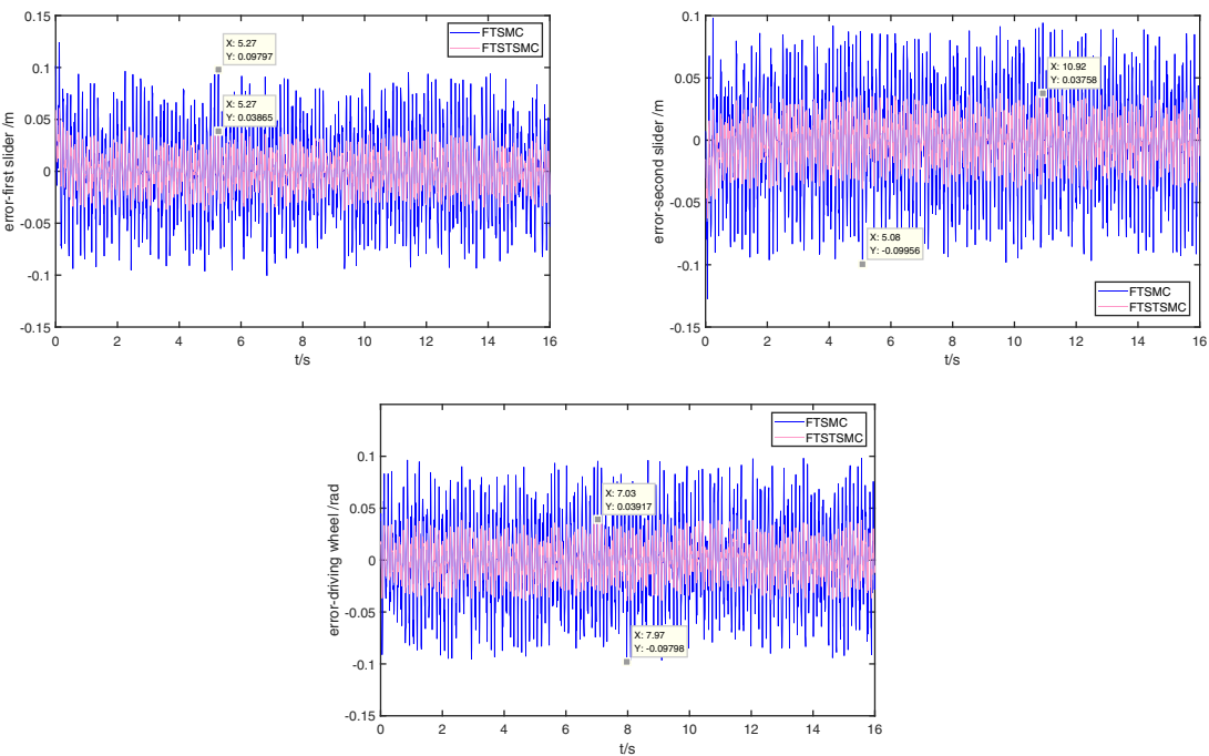
Figure 15. Experimental results of tracking errors for FTSTSCM and FTSTSMC.
