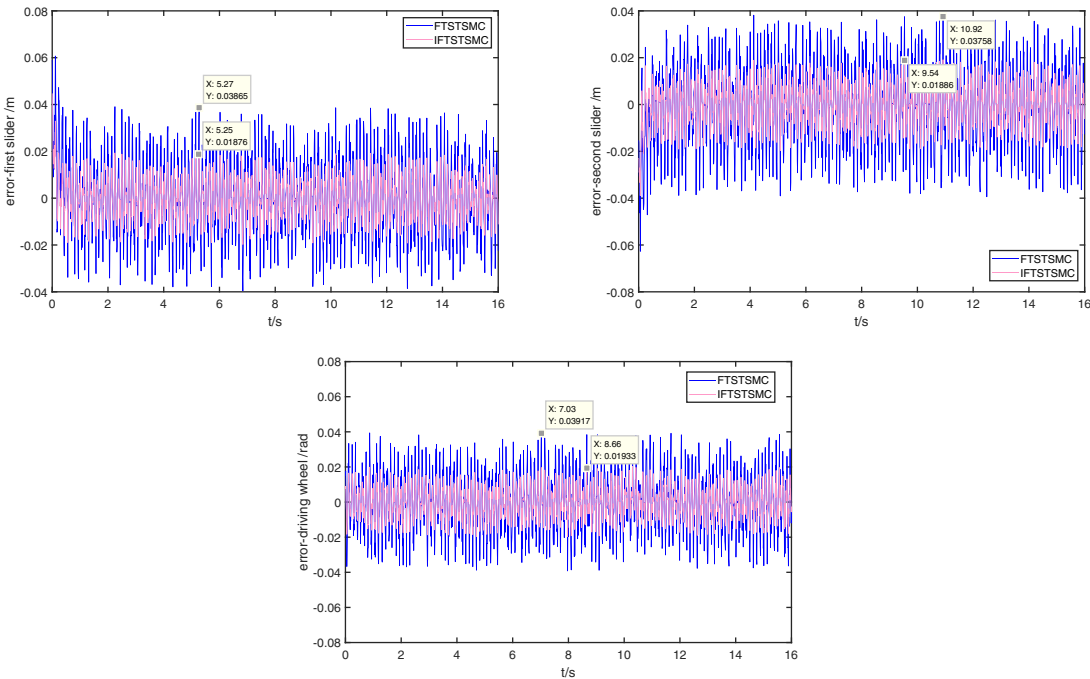
Figure 17. Experimental results of tracking errors for FTSTSMC and IFTSTSMC.
