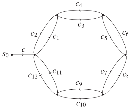
FIGURE 7. The graph G = L \cup c \subset M .
