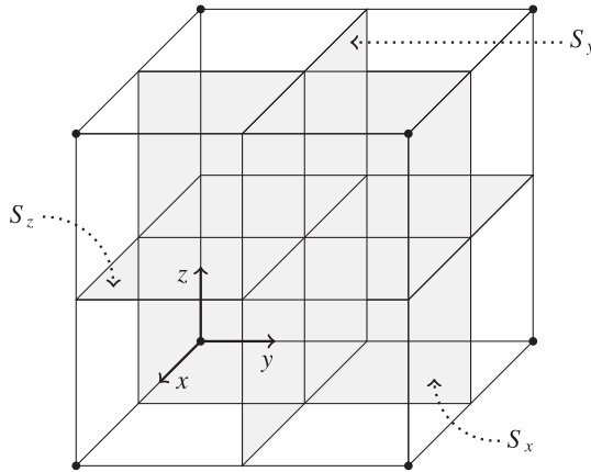
FIGURE 5. The cube Q with three distinguished squares.
