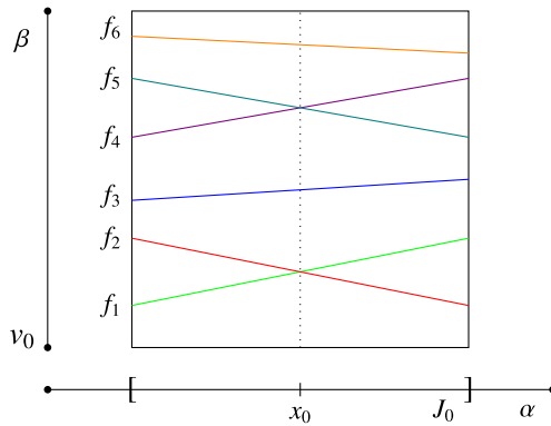
FIGURE 3. Maps with just a simple coincidence.
