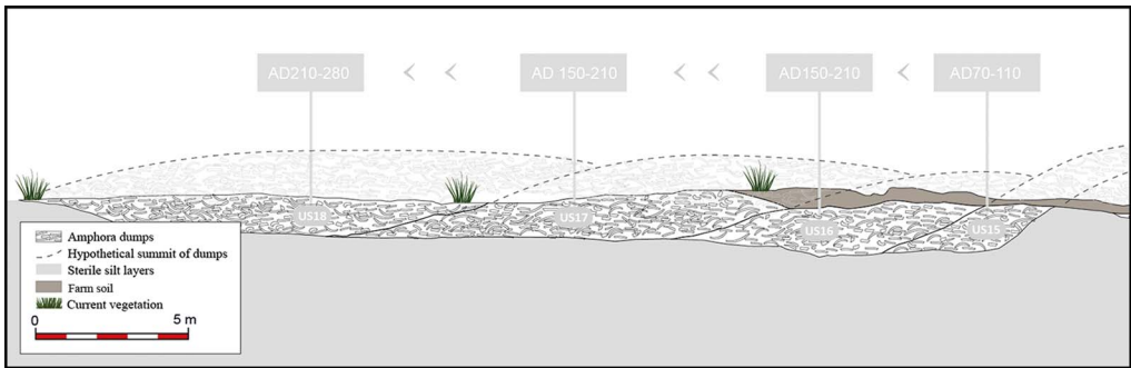
Figure 7. Cross section of the succession of amphora waster dumps at the workshop of El Sotillo (Almodóvar del Río, Córdoba) (figure by I. González Tobar).
