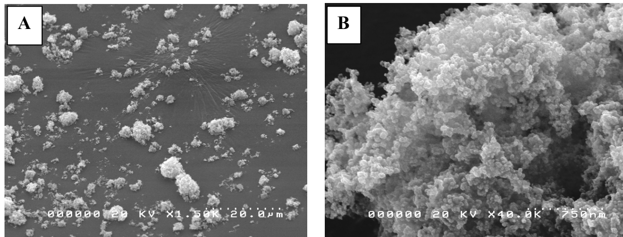
Fig. 3. A. The lower magnification micrograph of the \text{TiO}_2 nanoparticles shows a large distribution of micron scale agglomerates. B. At higher magnifications individual \text{TiO}_2 nanoparticles were observed in the larger agglomerates. To improve output of the nanocrystalline solar cell further processing of the \text{TiO}_2 powder will be needed to reduce particle sizes.
