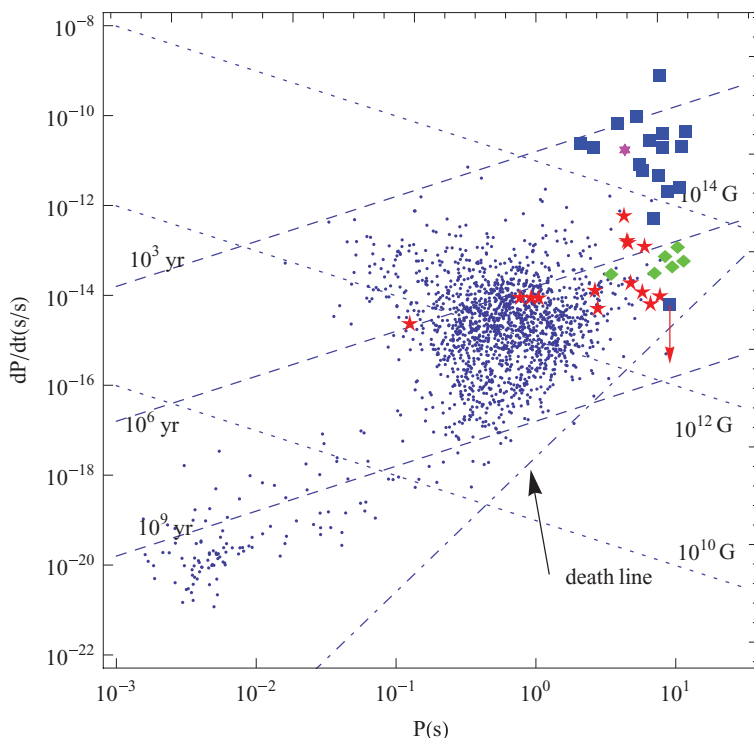
Figure 1. P - \dot{P} diagram. Squares are for AXPs and SGRs, the six-pointed-star is for the radio magnetar (from McGill online), diamonds for X-ray dim isolated neutron stars (XDINSs), stars for rotating radio transients (RRATs), and dots for normal pulsars (from the ATNF).
