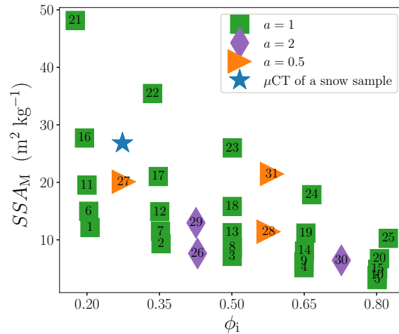
Fig. 2. The ice volume fraction \phi_i and the SSA SSA_M of the GRF ensemble. Each number corresponds to a GRF microstructure. For a comparison, \phi_i and SSA_M of a \mu CT image of a real snow sample that is presented in Fig. 3 are shown.
