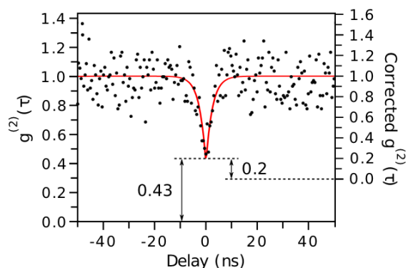
Figure 1. Cathodoluminescence time-auto-correlation function from a UV-emitting point defect in hBN. The dip at zero-delay is typical from an antibunching behavior, a signature of single photon emission. After [2].
