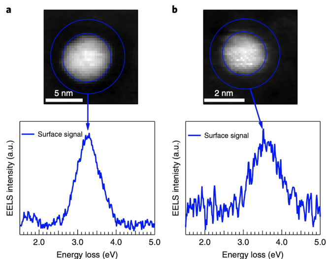
Figure 2. EELS signal coming from the surface of silver nanoclusters embedded in silicon oxide. The observed blue shift could be naively attributed to a quantum confined effect as the particle size decreases. A full quantum treatment shows that spill-out and quantum confinement should cancel due to the presence of the matrix, and no blue-shift is expected; this shift is most likely due to the change in matrix porosity due to electron irradiation. After [5].
