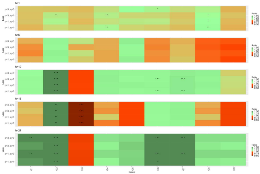
Figure 7. Heatmap for the score ratios (combined forecasts). Index: Wholesale. Method: Lasso, Benchmark: BM2.
