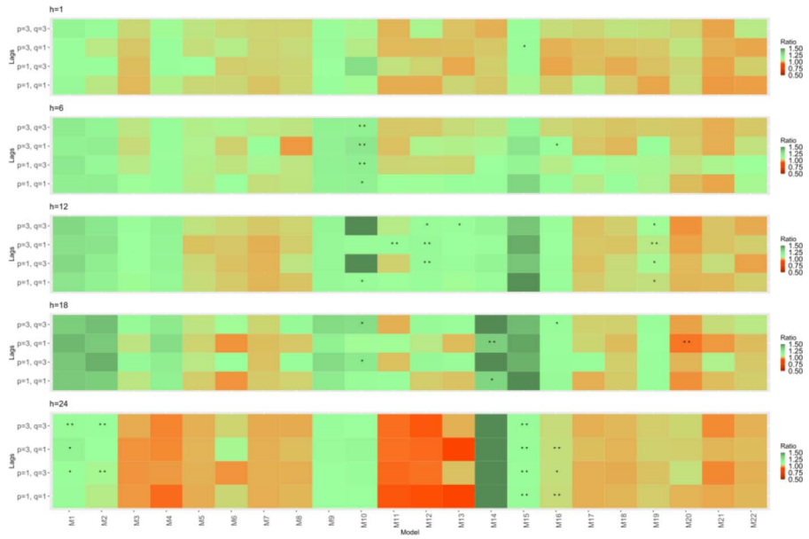
Figure 6. Heatmap for the score ratios. Index: Wholesale. Method: Lasso, Benchmark: BM2. Note: SR is the ratio between the RMSE of a given model and the one of the benchmark model BM2 (distributed lag model with the last three lagged month-on-month changes in wine prices as control variable). The stars in each cell are related to the p -values for the null hypothesis of equal predictability (test of Diebold and Mariano, 2002). ***, **, and * denote significance at the 1%, 5%, and 10% levels, respectively.
