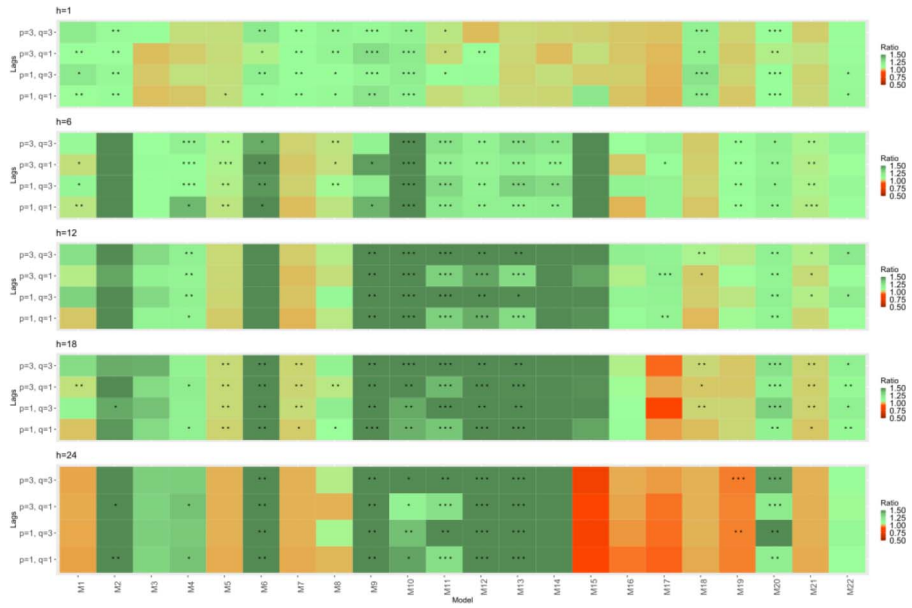
Figure 4. Heatmap for the score ratios. Index: Liv-ex Fine Wine 100. Method: Lasso, Benchmark: BM2. Note: SR is the ratio between the RMSE of a given model and the one of the benchmark model BM2 (distributed lag model with the last three lagged month-on-month changes in wine prices as control variable). The stars in each cell are related to the p -values for the null hypothesis of equal predictability (test of Diebold and Mariano, 2002). ***, **, and * denote significance at the 1%, 5%, and 10% levels, respectively.
