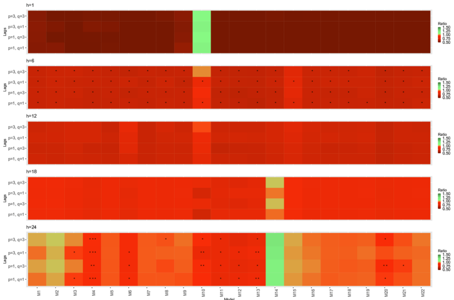
Figure 3. Heatmap for the score ratios. Index: Retail. Method: Lasso, Benchmark: BM1. Note: SR is the ratio between the RMSE of a given model and the one of the benchmark model BM1 (random walk in growth). The stars in each cell are related to the p -values for the null hypothesis of equal predictability (test of Diebold and Mariano, 2002). ***, **, and * denote significance at the 1%, 5%, and 10% levels, respectively.
