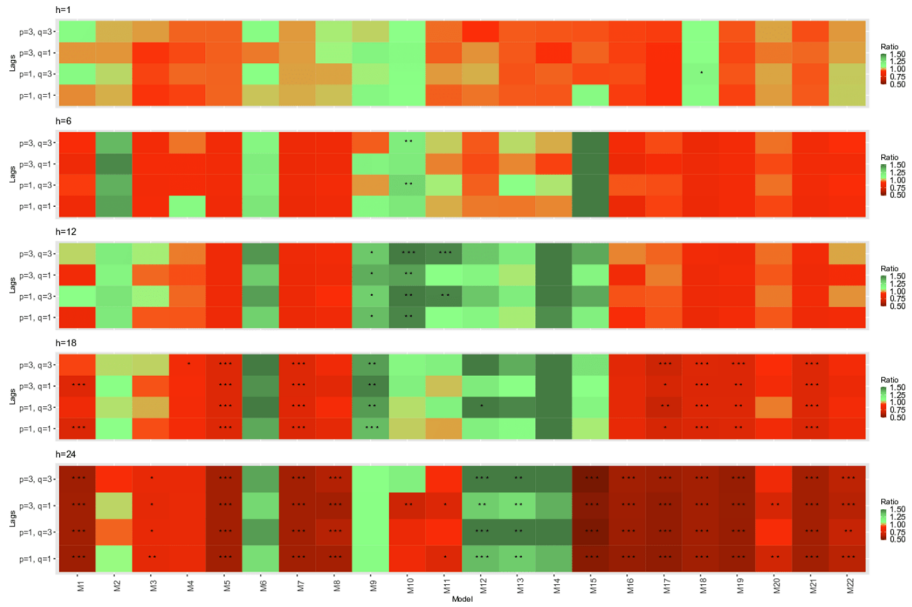
Figure 2. Heatmap for the score ratios. Index: Liv-ex Fine Wine 100. Method: Lasso, Benchmark: BM1. Note: SR is the ratio between the RMSE of a given model and the one of the benchmark model BM1 (random walk in growth). The stars in each cell are related to the p -values for the null hypothesis of equal predictability (test of Diebold and Mariano, 2002). ***, **, and * denote significance at the 1%, 5%, and 10% levels, respectively.
