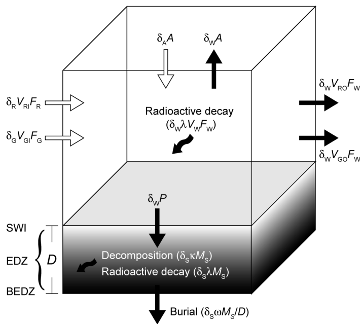
Figure 1 Two-component box model illustrating the mass budget of 14 C in a lacustrine sediment system. SWI: sediment-water interface; EDZ: early diagenesis zone; BEDZ: base of early diagenesis zone; D: thickness of early diagenesis zone.
