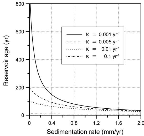
Figure 5 14 C reservoir age due to early diagenesis of OM plotted against sedimentation rate for 4 different decomposition rates.
