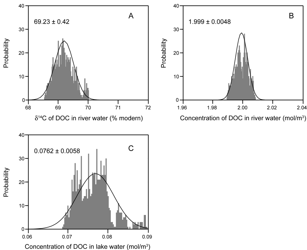
Figure 4 Markov chain Monte Carlo outputs of the posterior probability distribution of model parameters. Solid lines are the fits using a Gaussian probability distribution function. A) \delta^{14}\text{C} of DOC in river water; B) concentration of DOC in river water; and C) concentration of DOC in lake water.
