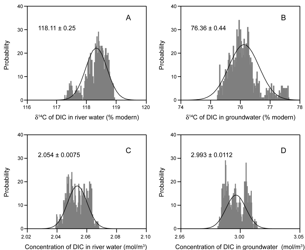
Figure 3 Markov chain Monte Carlo outputs of the posterior probability distribution of model parameters. Solid lines are the fits using a Gaussian probability distribution function. A) \delta^{14}\text{C} of DIC in river water; B) \delta^{14}\text{C} of DIC in groundwater; C) concentration of DIC in river water; and D) concentration of DIC in groundwater.
