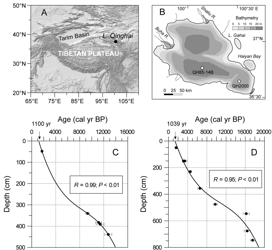
Figure 2 A) Shaded relief map of Lake Qinghai and the surrounding area; B) map showing the bathymetry of Lake Qinghai and the location of cores; C) age-depth model for Core QH85-14B (Kelts et al. 1989); D) age-depth model for Core QH2000 (Shen et al. 2005).
