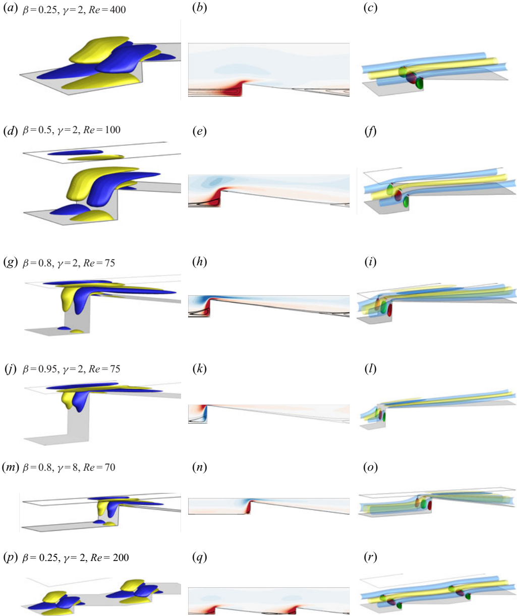
Figure 13. (a,d,g,j,m) Positive (blue) and negative (yellow) iso-surfaces of streamwise vorticity \hat{\omega}_x of the leading eigenmodes, (b,e,h,k,n) spanwise velocity ( \hat{w} ) contours overlaid with base flow streamlines and (c,f,i,l,o) positive and negative iso-contours of streamwise ( \hat{u} ) (represented as translucent surfaces) and transverse ( \hat{v} ) velocities (represented as opaque surfaces) of the leading mode. All the cases have a wedge angle of \tan(\phi) = 0.125 . The \hat{w} contours are shown in the linear scale at 20 equispaced levels between -0.001 (blue) and 0.001 (red). (p-r) Show the corresponding quantities as in (a-c) for a double-wedge case.
