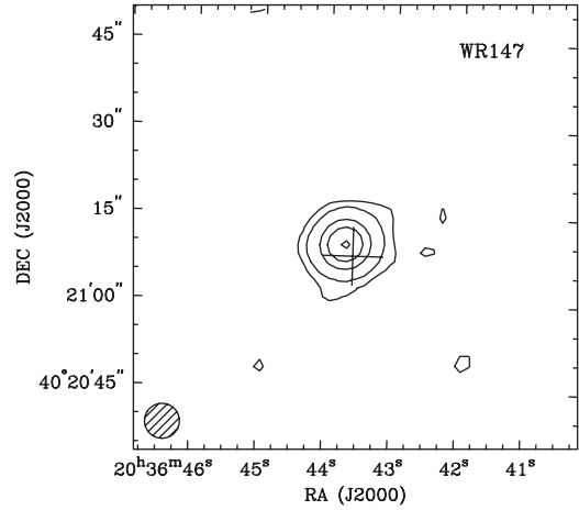
Figure 5. GMRT image of the system WR 147 at 610 MHz. The contour levels are -0.24, 0.24 (=3\sigma), 2, 5, 10, and 18 mJy per beam. Hatched, the synthesised beam. Cross hair: optical position of the system (see Table 1).
