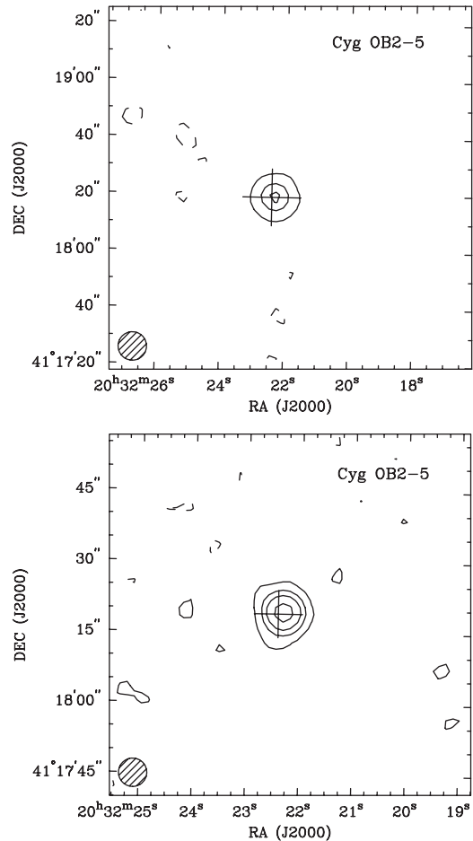
Figure 6. GMRT images of the system Cyg OB2-5. Top panel: at 325 MHz; contour levels of -0.7, 0.7 (=3\sigma), 3, and 5 mJy per beam. Bottom panel: at 610 MHz; contour levels of -0.15, 0.17 (=2\sigma), 0.75, 1.5, and 3 mJy per beam. Hatched, the synthesised beam. Cross hair: optical position of the system (see Table 2).
