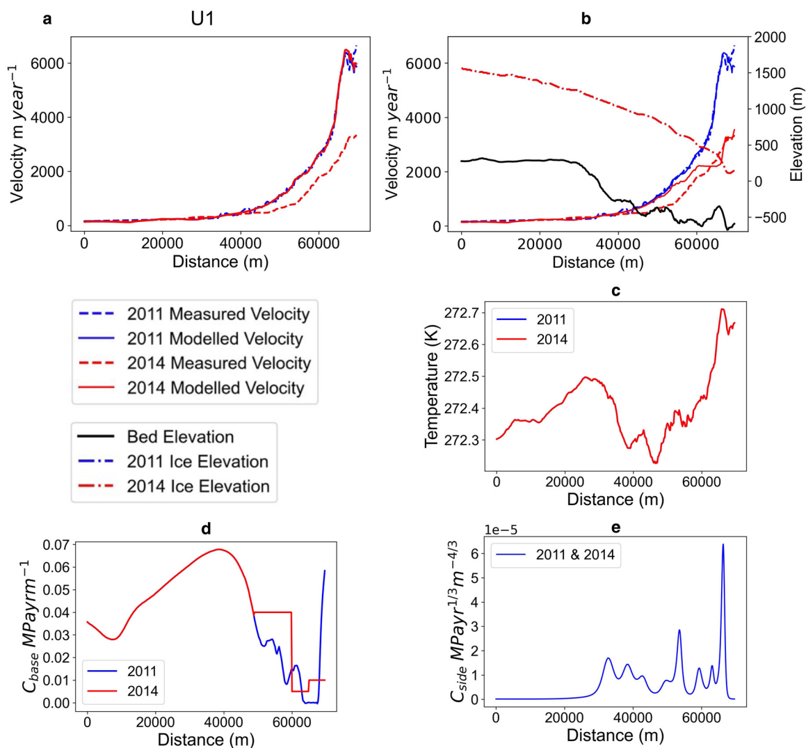
Figure 7. U1 model inputs and ice-flow speeds. (a) U1 measured and modeled velocity using the same drag inputs ( C_{base} , C_{side} ) over time. (b) U1 measured and modeled velocity in 2011 and 2014 using modified basal drag coefficient, along with ice-surface elevation and bed depth. (c) U1 basal temperature in 2011 and 2014. (d) U1 basal drag inversion output ( C_{base} ) in 2011 and manipulated drag in 2014. (e) U1 sidewall drag inversion output ( C_{side} ) used in both model runs. The flowline starts at 0 m at the upper glacier and approaches the terminus point toward 75 km.
