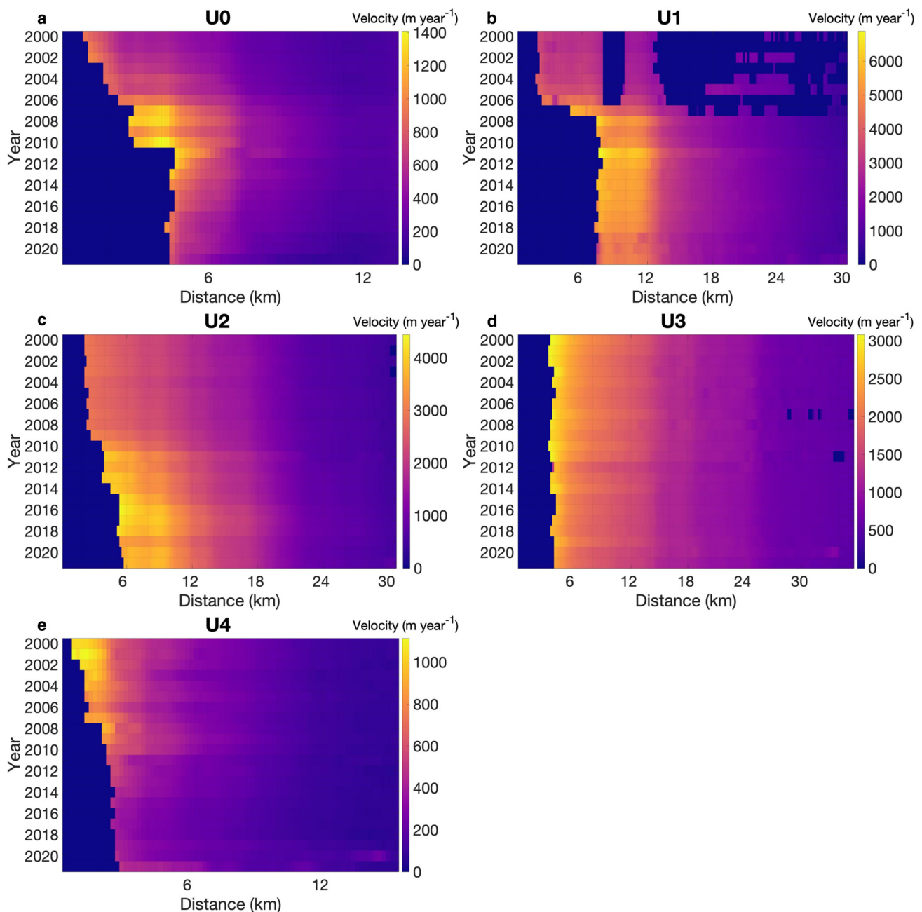
Figure 2. Upernavik flowline summer velocities. (a–e) Hovmöller summer velocity diagrams from 2000 to 2021 for the flowlines of U0–U4, respectively, ending at the terminus position in each year, determined using data from PROMICE (Andersen and others, 2019). Velocity scales vary between outlets. All velocity data from 2000 to 2018 are from ITS_LIVE velocity mosaics and from 2019 to 2021 the data are from stacked GoLIVE velocities (Gardner and others, 2019; Scambos and others, 2016).
