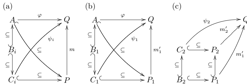
Figure 3. The mediating homomorphism.
