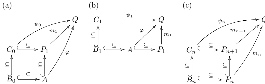
Figure 2. Three commuting diagrams.
