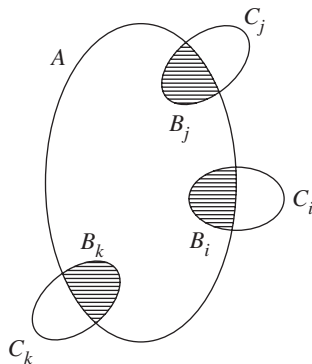
Figure 1. A rooted multi-amalgam.
