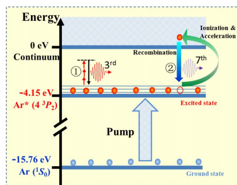
Figure 5. The physical picture of the 3rd and the 7th harmonic generation from the excited argon atoms.
