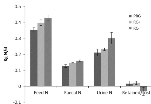
Figure 2 Nitrogen balance (kg/day) in cattle offered the three experimental silages in experiment 2. PPO = polyphenol oxidase; RC+ = high PPO red clover silage; RC- = low PPO red clover silage; PRG = perennial ryegrass silage.
