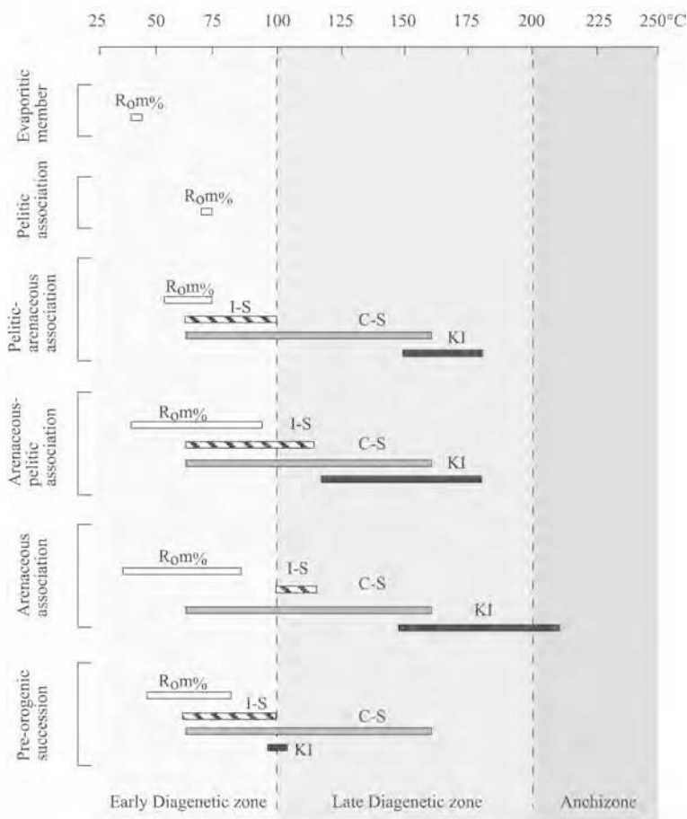
Figure 7. Temperature ranges derived from organic and inorganic thermal parameters. Note that KI-derived temperatures for the Laga Fm. do not match other ranges because the 10 Å phases come from either metamorphic or late diagenetic rocks. R o,m %-derived temperatures for the Laga Fm. are generally lower than those calculated from mixed-layer clay minerals (see text for explanation). They refer to minimum and maximum R o,m %-derived values without considering the standard deviation of each sample.
