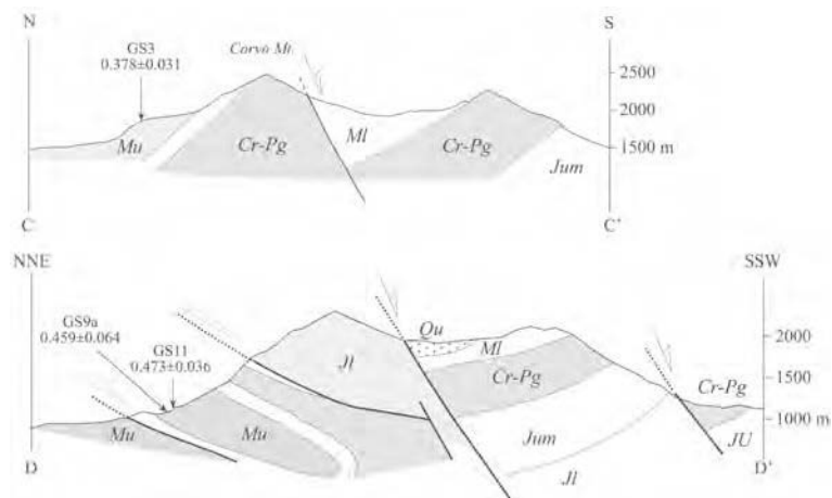
Figure 9. Cross-sections showing the structural setting of the Gran Sasso thrust belt and R_{0,m}\% samples (see Figure 1 for locations of the C–C' and D–D' cross-sections). Observe the decrease in shortening from the eastern to the western part of the range (redrawn and modified by Ghisetti and Vezzani, 1986; D'Agostino et al. , 1998; D'Agostino and Corrado, 1999). Legend: JI = Lower Jurassic; Jum = Upper–Middle Jurassic; Cr–Pg = Cretaceous–Paleogene; MI = Lower Miocene; Mu = Upper Miocene (comprising pelitic lithology association); Qu = Quaternary.
