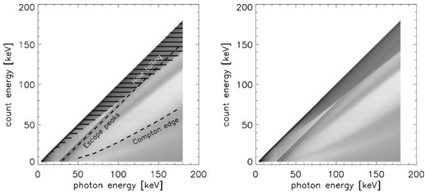
Figure 1. Left panel: DRM of Caliste SO with marked hole tailing, escape peaks, and Compton edge. Right panel: DRM from Geant4 simulations without marked features.
