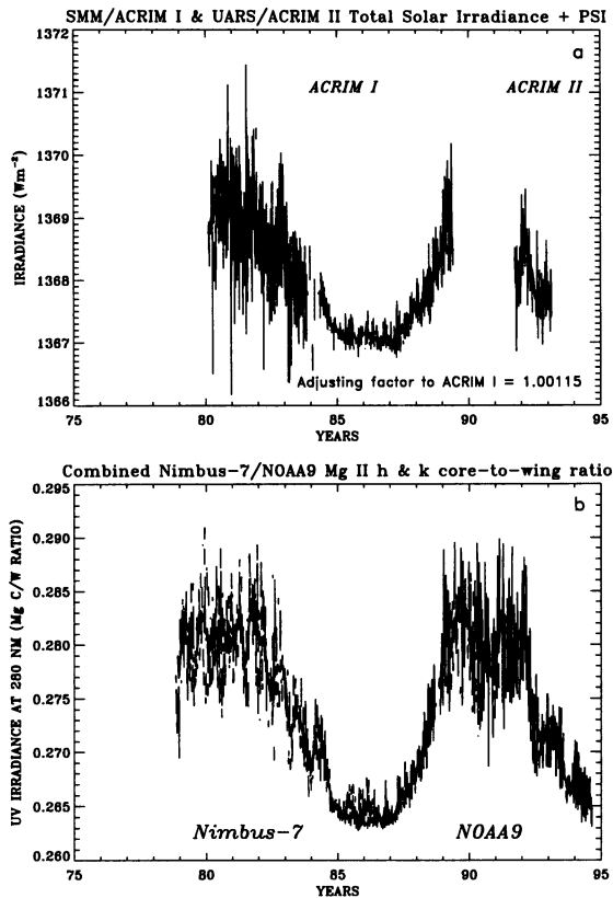
Figure 3. Total solar irradiance corrected for sunspot darkening is presented in Fig. 3a. The combined Nimbus-7/SBUV1 and NOAA9/SBUV2 Mg c/w ratio is shown in Fig. 3b.
