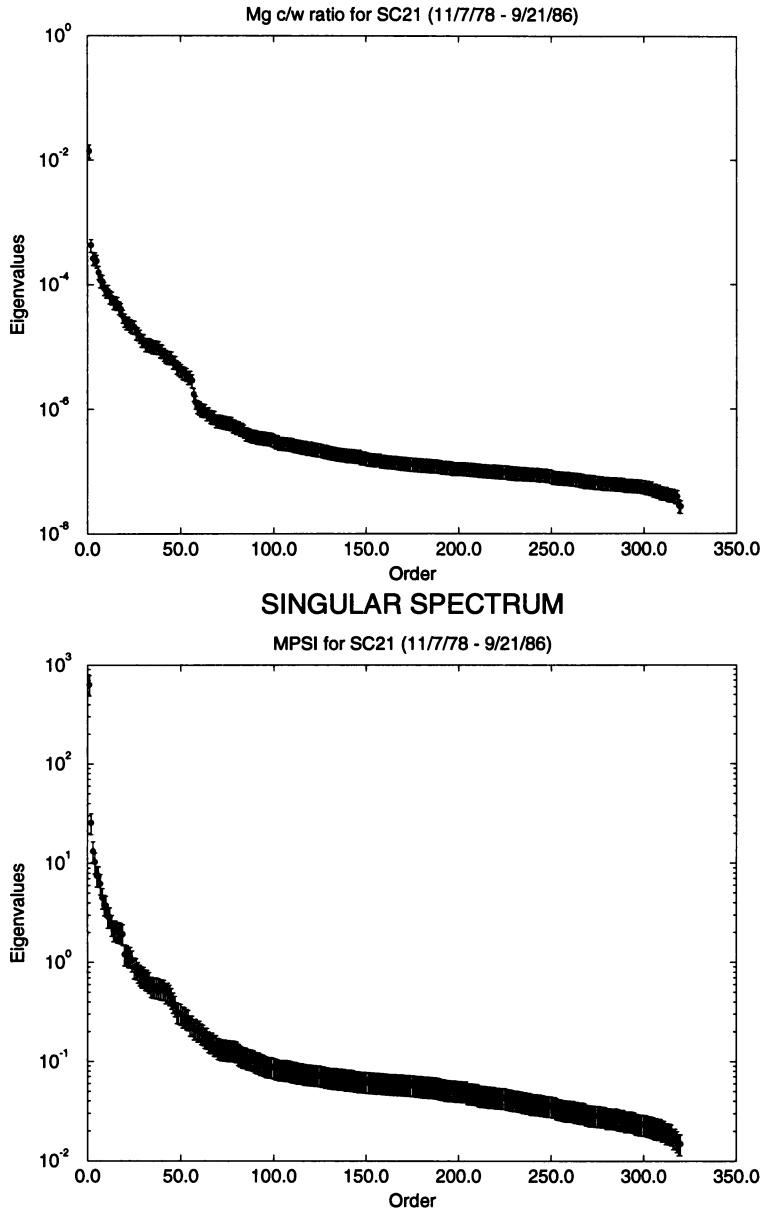
Figure 6. The Singular Spectra of the Mg c/w ratio (upper panel) and MPSI (lower panel) for solar cycle 21.
