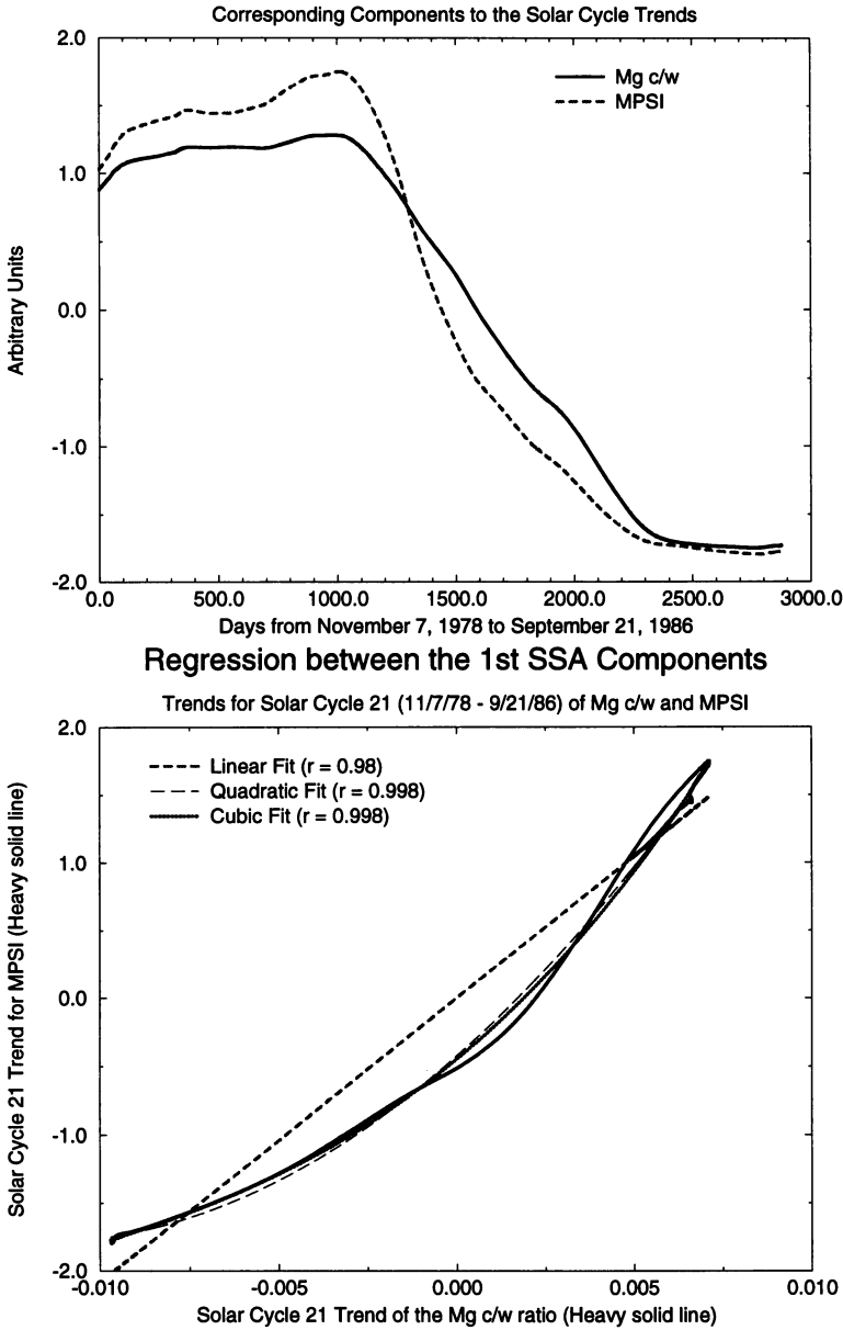
Figure 7. The upper panel shows the 1st RCs of the Mg c/w ratio (heavy solid line) and MPSI (heavy-dashed line) for solar cycle 21. The lower panel shows the correlation between the two RCs.
