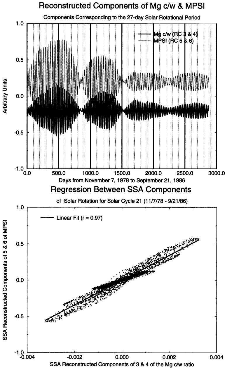
Figure 8. The 3rd and 4th Reconstructed Components of the Mg c/w ratio (heavy line) for solar cycle 21 are presented on the upper panel. These RCs represent the 27-day solar rotational component in the signal. The correlation between these components is shown on the lower panel.
