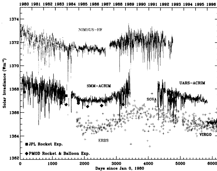
Figure 1. The time series of various space-borne irradiance experiments are presented (from Fröhlich, 1997). Fig. 1 has been provided for this paper by courtesy of the SOHO/VIRGO Science Team.
