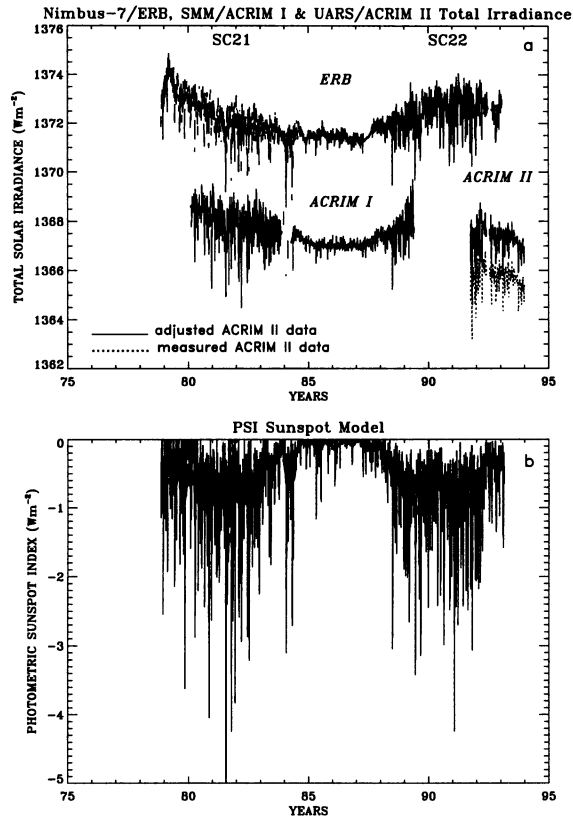
Figure 2. The Nimbus-7/ERB, SMM/ACRIM I and UARS/ACRIM II total irradiance data are shown in Fig. 2a. Fig. 2b shows the PSI model calculated by Fröhlich et al. (1994).
