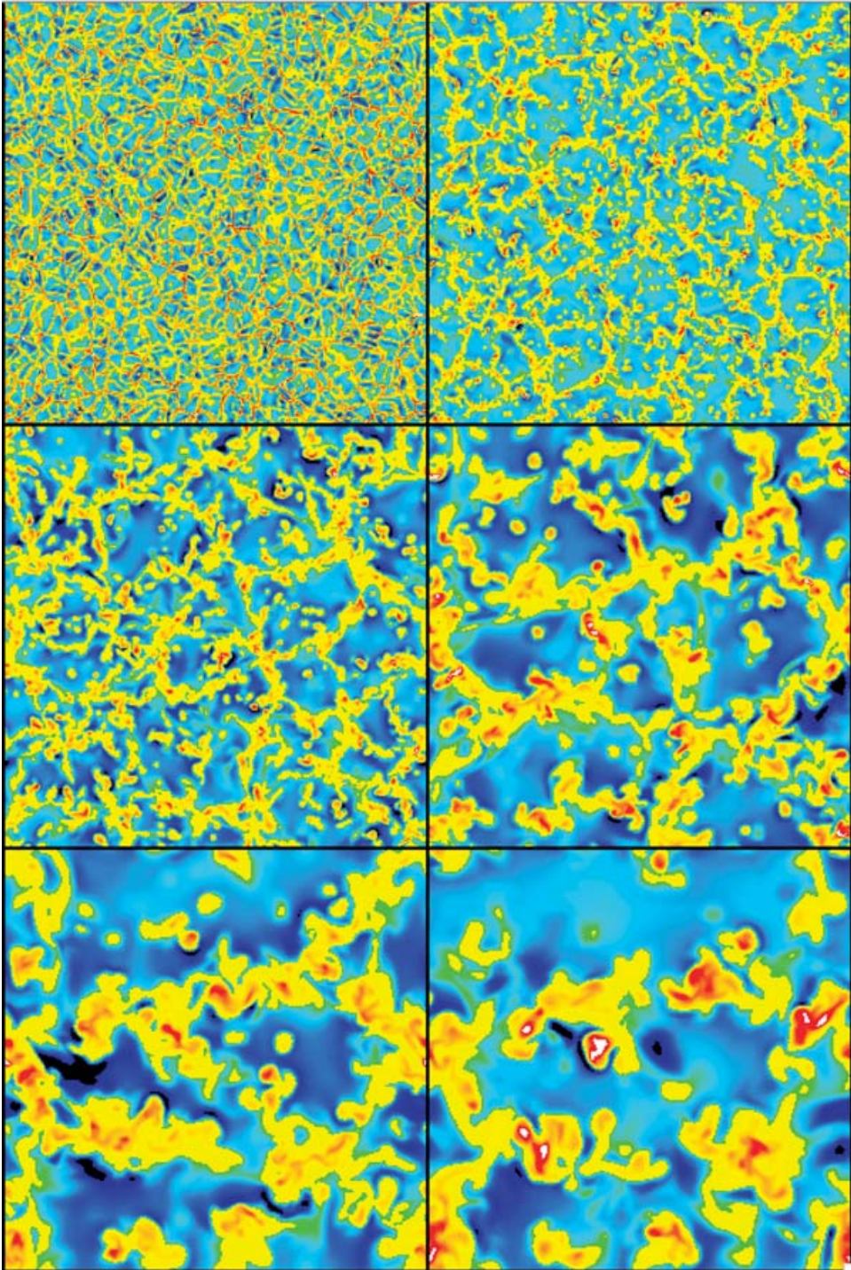
Figure 4. Vertical velocity in horizontal slices at increasing depth. Going from the surface at the top left across and down at depths of 2, 4, 8, 12 and 16 Mm. Red and yellow (light gray) are downflows, blue and green (dark gray) are upflows. Each depth is scaled separately.
