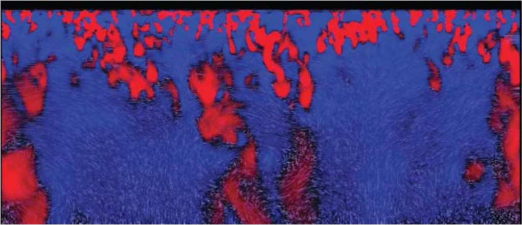
Figure 3. Fluid velocity in vertical plane. Width is 48 Mm and depth 20 Mm. Light gray (Red) are downflows and dark gray (blue) are upflows. Streaks are streamlines. At the top of the convection zone the structures are small granules. The size of the structures increases gradually with increasing depth as the diverging upflows either halt some of the downflows or sweep them into the larger downflows.
