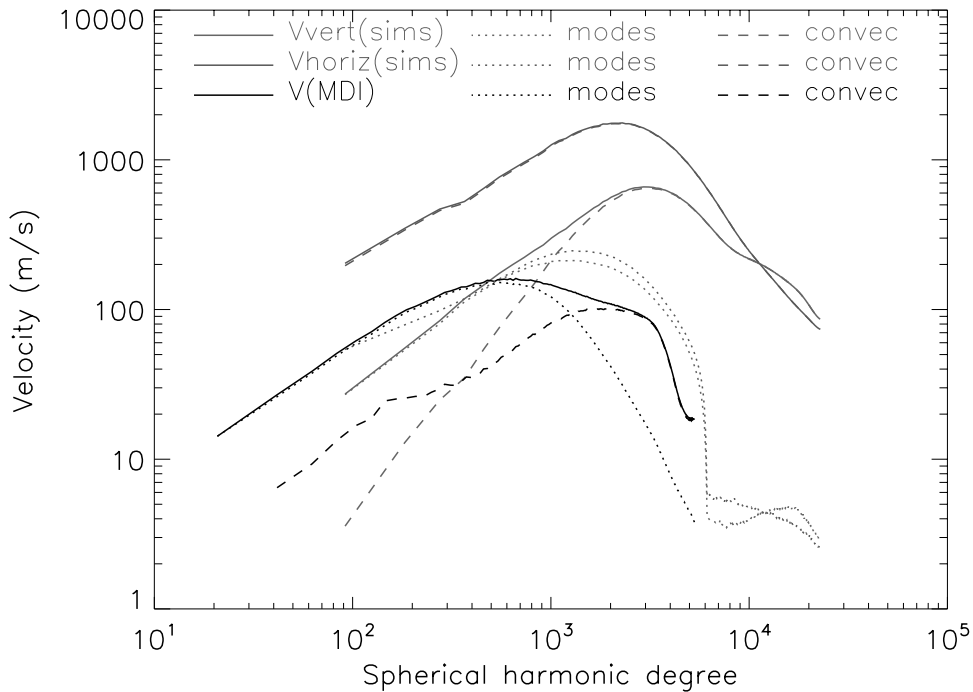
Figure 6. Velocity spectra for the simulation and MDI observations, separated into convective (dashed lines), oscillatory (dotted lines) and total (solid lines) components. The dark or red set is for the MDI high resolution velocity observations. The light or green set is for the vertical simulation velocities. The medium grey or blue set is for the horizontal simulation velocities. The oscillatory signal is negligible in the horizontal velocity but dominates the vertical velocity and MDI Doppler velocity on large scales ( \ell \leq 1000 ). The horizontal velocity is almost purely convective.
