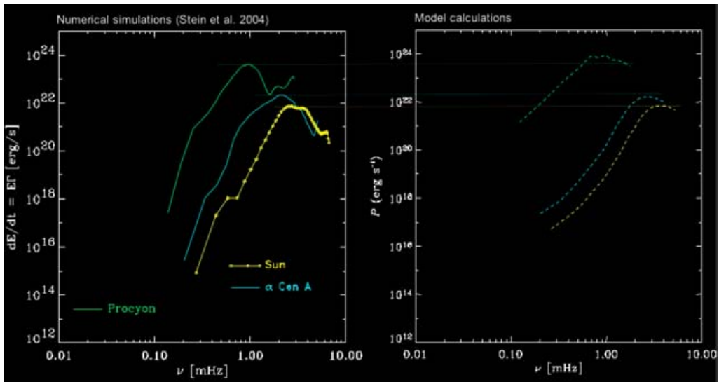
Figure 1. Comparison of numerical and analytic p -mode excitation rates for three stars: the Sun, \alpha Cen A and Procyon (upper curve) using Houdek’s analytic expression.
