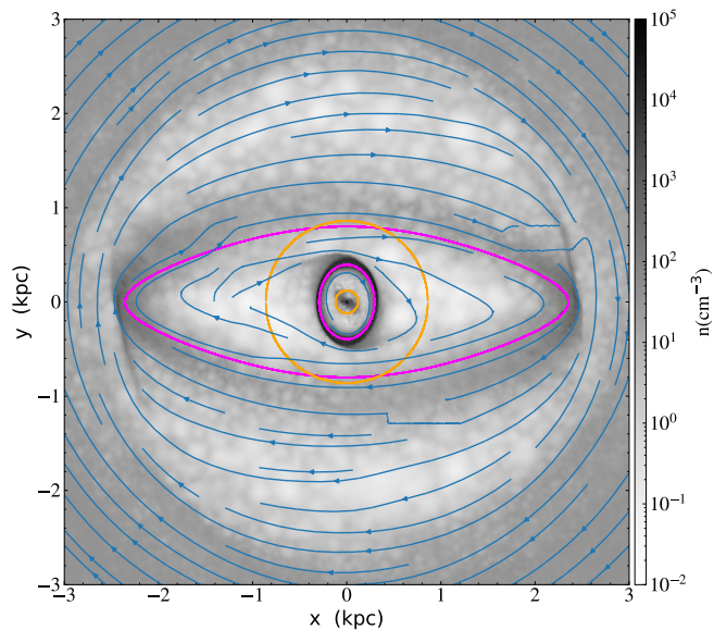
Figure 2. Density map at t = 2000 Myr. The magenta lines correspond to two orbits from the x_1 (outer line, E_j = -0.444 \text{ kpc}^2/\text{Myr}^2 ) and x_2 family (inner line, E_j = -0.486 \text{ kpc}^2/\text{Myr}^2 ). The orange circles denote the positions of the iILR and the oILR.
