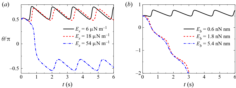
Figure 14. Instantaneous inclination angle for different (a) shear moduli and (b) bending moduli at the phase difference \varphi = 30\pi/64 . The black line shows the result at the shear modulus E_s = 6 \mu\text{N m}^{-1} and the bending modulus E_b = 0.6 \text{ nN nm} .
