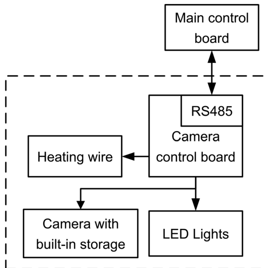
Fig. 14. Block diagram of the camera system.
