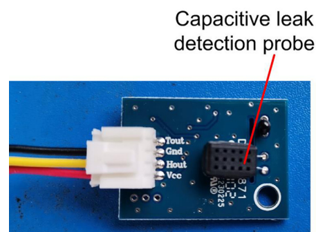
Fig. 13. Capacitive relative humidity sensor for leak detection.
