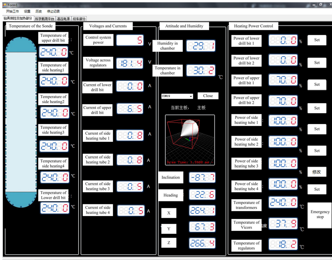
Fig. 18. Control screen of RECAS monitor and heating control. It includes four parts, namely, the temperature of the sonde, voltages and currents, attitude sensor and humidity, and heating power control, from left to right.
