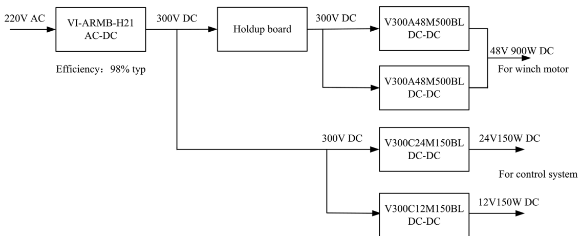
Fig. 3. Block diagram of power supply for the downhole control system.
