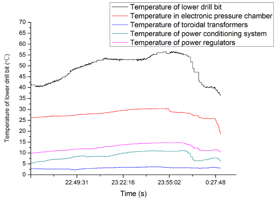
Fig. 27. Temperature of key components during a downward penetration.
