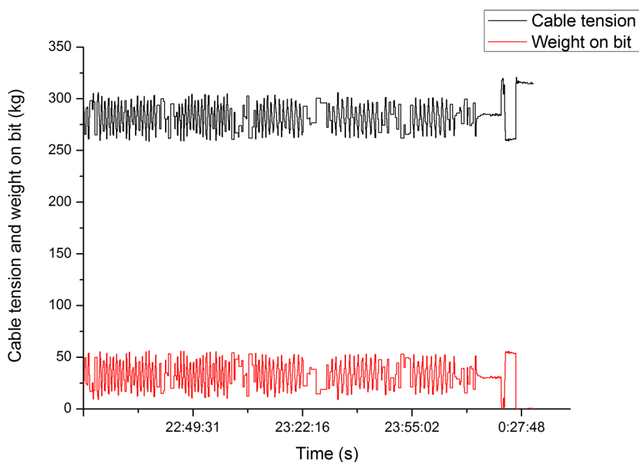
Fig. 26. Cable tension and WOB during a downward penetration.
