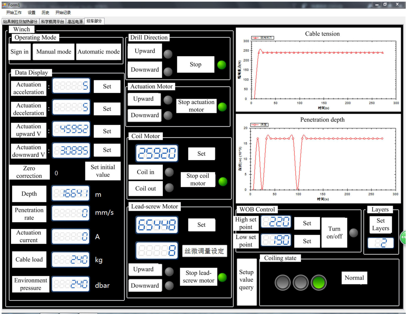
Fig. 19. Control screen of downhole winch system, including parameter settings and status display of the winch system and the control over the winch system. The cable tension and penetration depth are displayed in dynamic curves.
