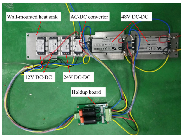
Fig. 4. Assembled power supply for the downhole control system.
