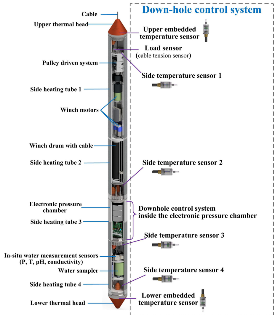
Fig. 5. Overall structure of RECAS-200 and location of the proposed downhole control system.
