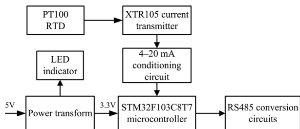
Fig. 8. Block diagram of self-developed temperature sensors.
