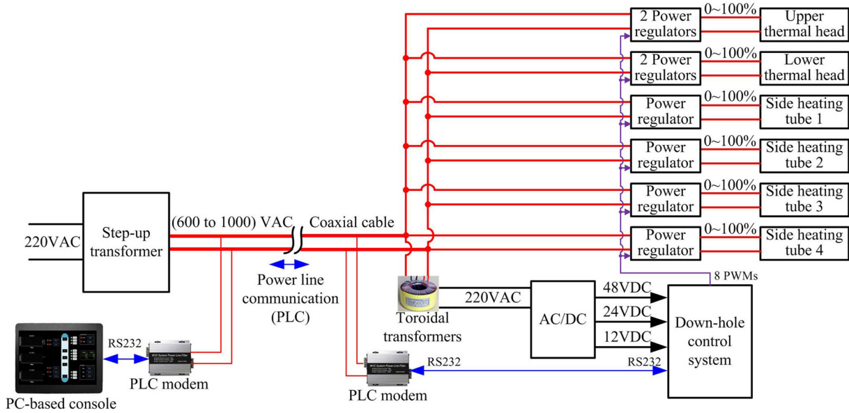
Fig. 2. Block diagram of PTCS.
