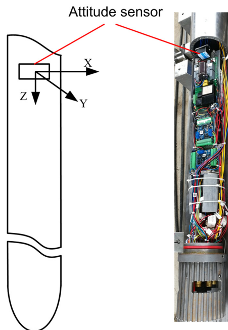
Fig. 12. Installation of the attitude sensor.
