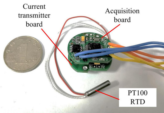
Fig. 10. Internal elements of a temperature sensor.
