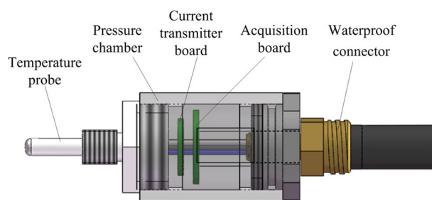
Fig. 9. Structure of self-developed temperature sensors.
