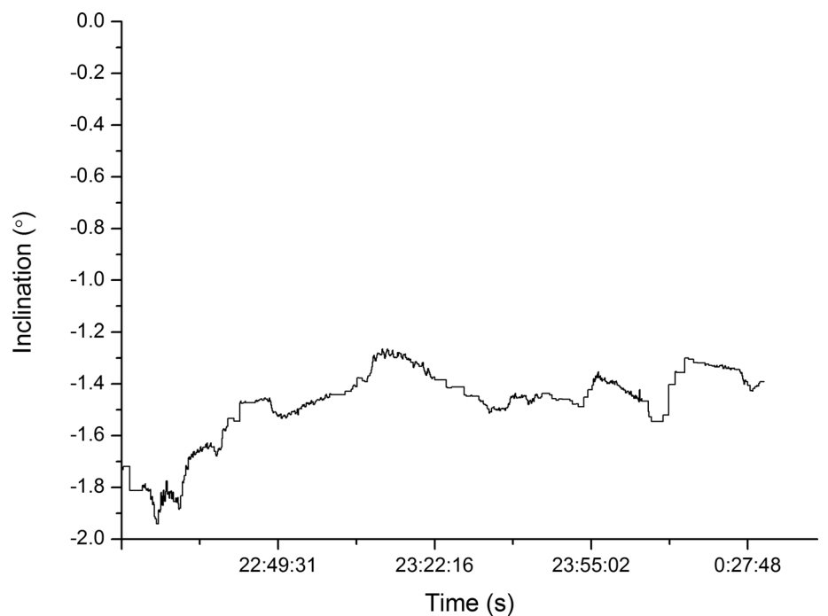
Fig. 28. Inclinations of the probe during a downward penetration.
