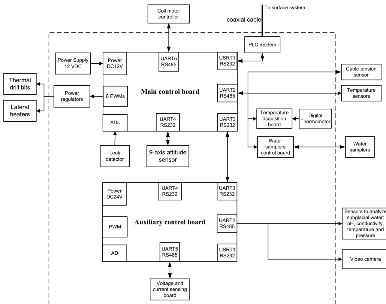
Fig. 6. Block diagram view of the downhole control system.
