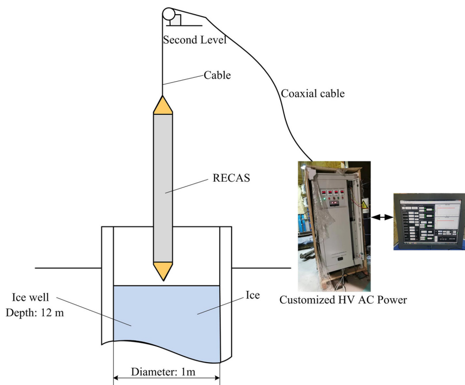
Fig. 23. Experimental set up of RECAS-200 prototype tests.
