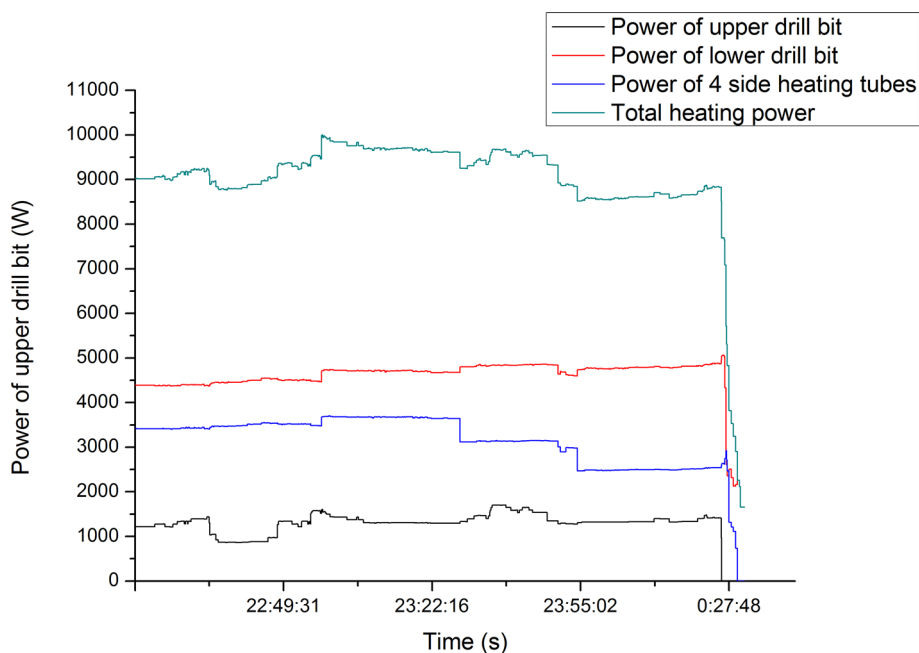
Fig. 25. Heating power during a downward penetration.
