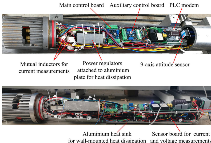
Fig. 7. Electronic components in the pressure chamber: (a) top view; (b) side view.
