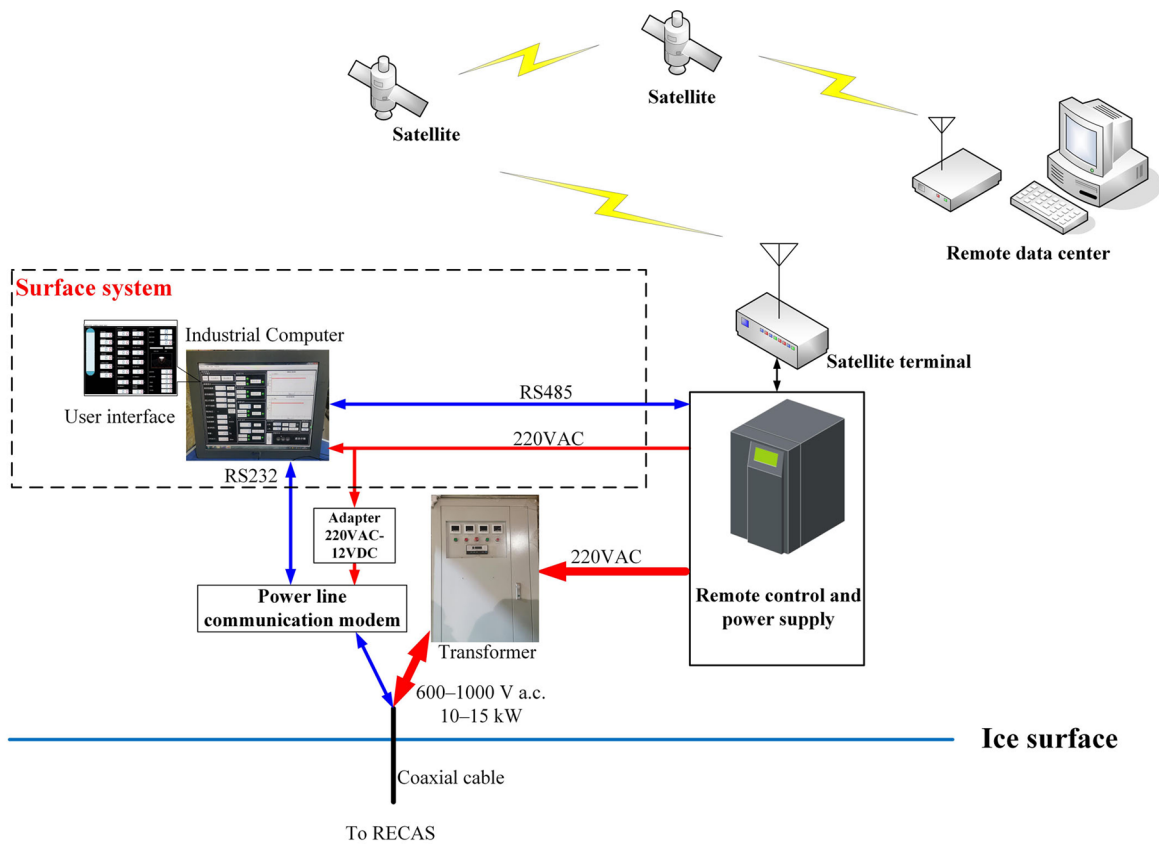
Fig. 17. Block diagram of the surface system.
