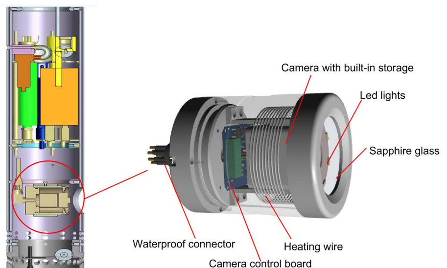
Fig. 15. Structure of the camera system with built-in storage.
