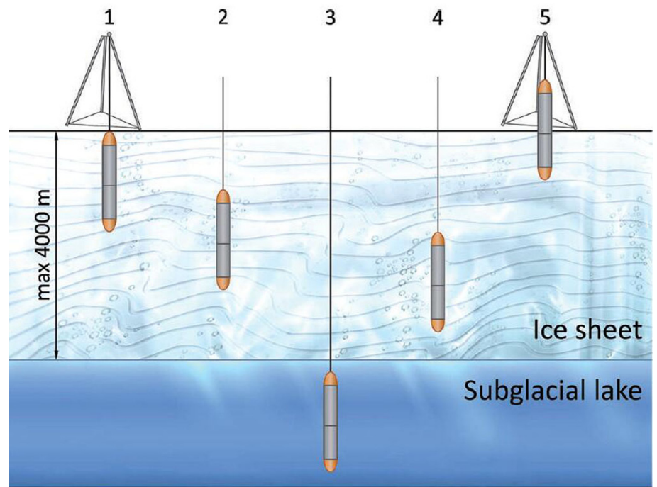
Fig. 1. Concept of RECAS and its workflow proposed by Talalay and others (2014).
