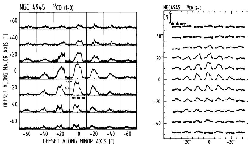
The spectra in the nuclear area in the CO(1-0) and CO(2-1) transitions
