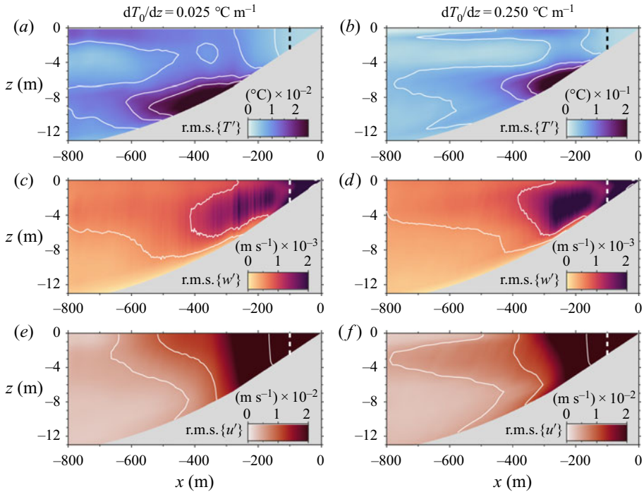
Figure 4. Time and along-shore root-mean-square (3.1) (a,b) temperature perturbation r.m.s.\{T'\}(x, z) with white contour intervals of 0.005 and 0.05\text{ }^\circ\text{C} in (a) and (b), respectively; (c,d) vertical velocity r.m.s.\{w'\} with white contours at \{0.5, 1\} \times 10^{-3}\text{ m s}^{-1} ; and (e,f) cross-shore velocity r.m.s.\{u'\} with contours at \{0.5, 1, 5\} \times 10^{-2}\text{ m s}^{-1} . Panels (a,c,e) have dT_0/dz = 0.025\text{ }^\circ\text{C m}^{-1} and correspond to panels (a,d,g,j) in figure 3; and panels (b,d,f) have dT_0/dz = 0.25\text{ }^\circ\text{C m}^{-1} , corresponding to panels (c,f,i,l) in figure 3. Note the approximate factor of 10 change in colour scale between (a) and (b). The L_{SZ} = 100\text{ m} wide surf zone is delimited with a vertical dashed line, and the bottom is grey.
