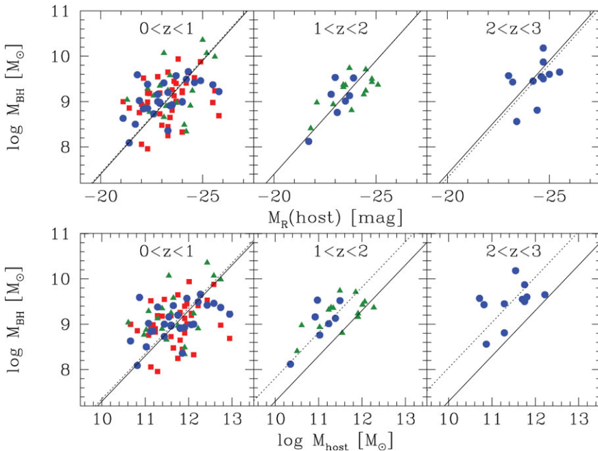
Figure 1. The M_{\text{BH}}-L_{\text{host}} and M_{\text{BH}}-M_{\text{host}} relations in three redshift bins. Squares, triangles and circles mark quasars in which M_{\text{BH}} is derived from \text{H}\beta , \text{Mg II} , and \text{C IV} , respectively. The solid line is the Bettoni et al. (2003) relation ( upper panels ) or M_{\text{BH}}/M_{\text{host}} = 0.002 ( lower panels ). The dotted line is the best fit to the data, assuming the slope of the rest-frame relations. Clear evolution is apparent in the M_{\text{BH}}-M_{\text{host}} relationship as a function of redshift.
