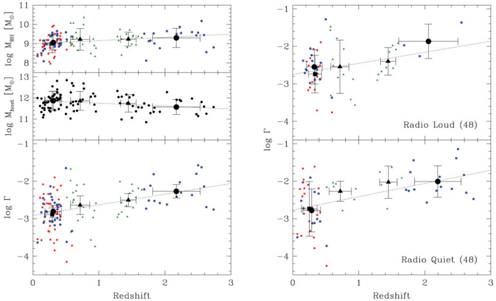
Figure 2. Left: The redshift dependence of M_{\text{BH}} ( top panel ), M_{\text{host}} ( middle panel ), and \Gamma ( bottom panel ). Symbols are as in Figure 1. The best linear fits, and the average points with rms as error bars of the H \beta (big square), the low- and high- z C IV (big circles) and the Mg II data with redshift z < 1 and z > 1 (big triangles) are shown. Right: The redshift dependence of \Gamma for radio-loud ( top panel ) and radio-quiet quasars ( bottom panel ).
