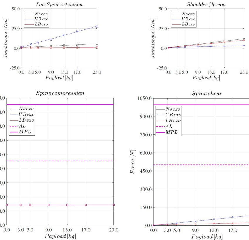
Figure 5. Joint torque and force - neutral posture with and without exoskeleton
