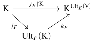
FIGURE 1. Factoring ultrapower embeddings with K .
