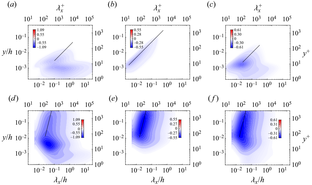
Figure 5. The premultiplied streamwise wavenumber spectra for dissipation from (a–c) DQLA and (d–f) DNS for the (a,d) streamwise, (b,e) wall-normal and (c,f) spanwise components at Re_\tau \approx 5200 . Contour levels are separated by 1% of the maximum value up to 10% of the maximum, and then in increments of 10%. The solid lines are y/\lambda_x = 0.03, 0.5 and 0.1 , and y^{1/4}/\lambda_x = 13, 20 and 20 for streamwise, wall-normal and spanwise components in the DQLA and DNS, respectively.
