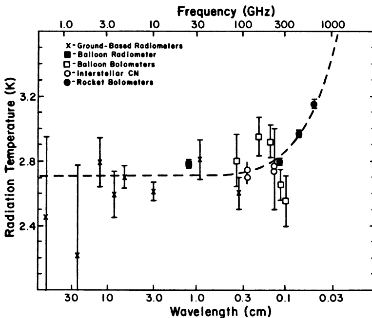
Fig. 1. Recent Measurements of the CMR Temperature.
