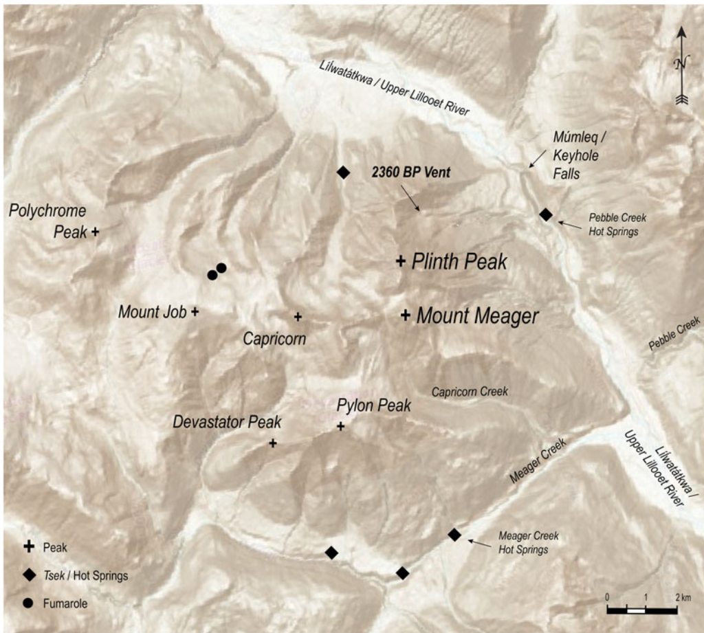
Figure 2. Topographic map indicating current peaks of the Mount Meager Complex.
