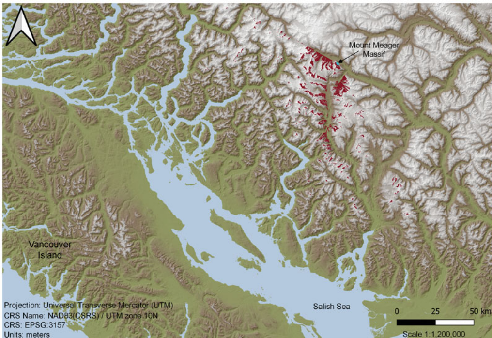
Figure 5. Viewshed analysis from current highest viewpoint at 2,680 MASL. Note: no visibility of the Salish Sea is possible.
