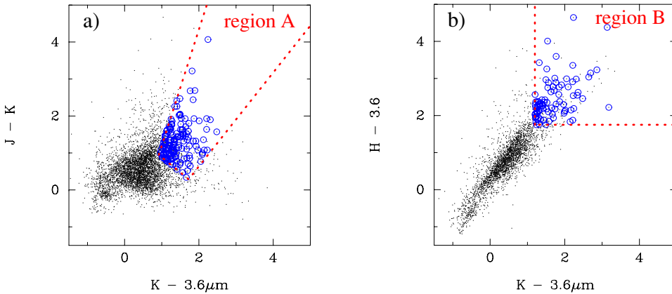
Figure 1. The color indices for the K_s -selected galaxies from the GOODS sample. Two alternative methods for selecting high redshift post-starburst galaxies using near- and mid-infrared colors. a) J-K vs. K_s - 3.6\mu\text{m} : the area inside the wedge outlined by the red line contains z > 5 post-starburst and dusty starburst galaxies. The selected candidates (shown as circles) will also contain dusty starburst systems at redshifts z \approx 2-8 . b) H-3.6\mu\text{m} vs. K-3.6\mu\text{m} : the area above and to the right of the red line contains z > 5 post-starburst and dusty starburst galaxies.
