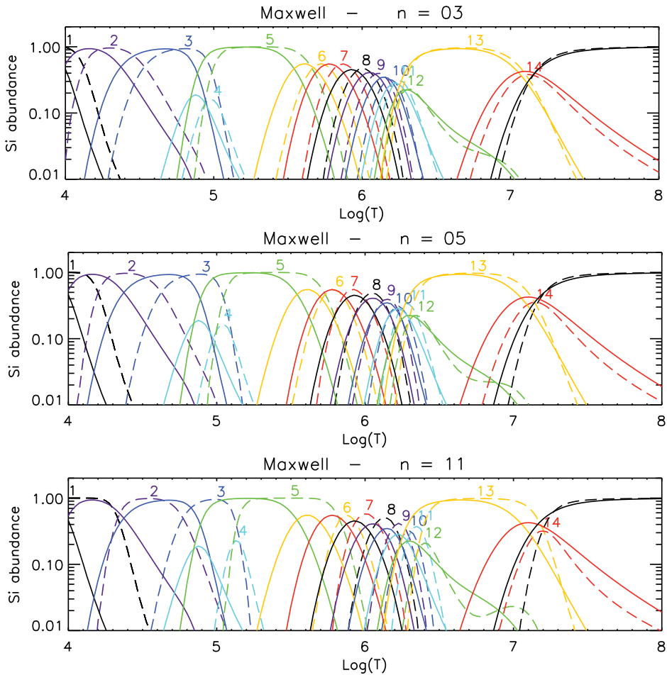
Figure 2. The ionization equilibrium for the Maxwellian (full lines) and n -distributions with different n (dashed lines) for the silicon in the temperature range 10^4 - 10^8 K. The same color corresponds to the same ions.
