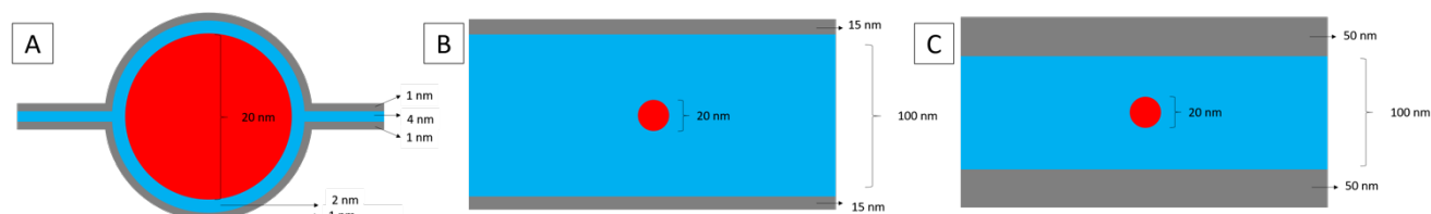
Figure 1. Experimental setup for A) GLC and B, C) Fluid cell STEM experimentation.
