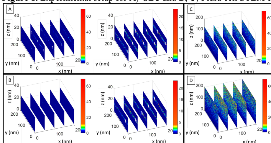
Figure 2. Monte Carlo simulation results for the energy deposition for 1) GLC-STEM at 80kV, 2) GLC-STEM at 200 kV, 3) Fluid cell-STEM with 15 nm thick \text{Si}_3\text{N}_4 window and 4) Fluid cell with 50 nm thick \text{Si}_3\text{N}_4 window (energy unit: \text{eV}/\text{nm}^3 ).
