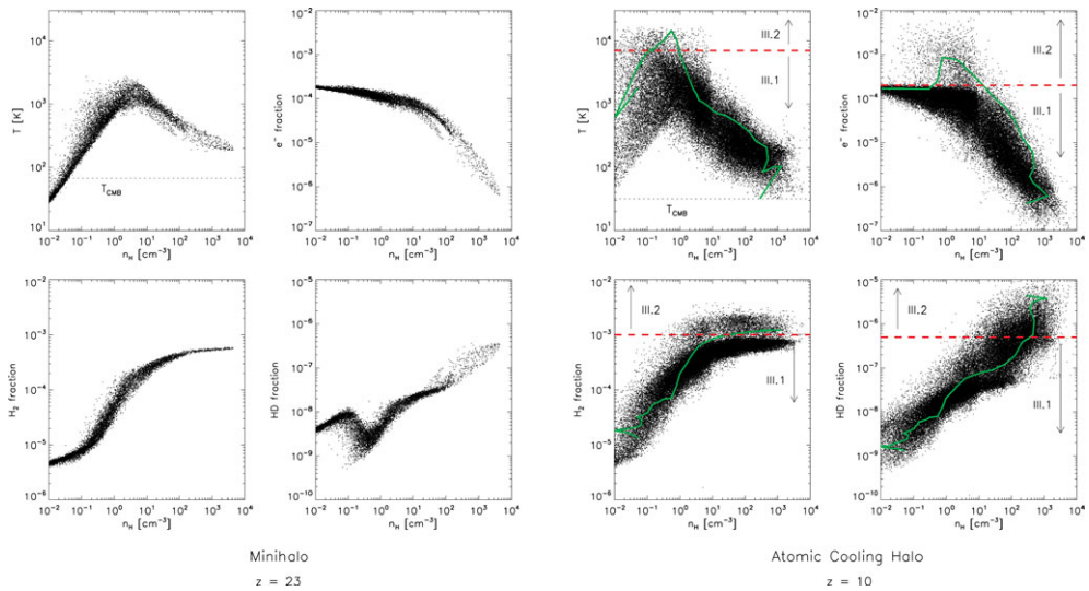
Figure 2. The phase-space distribution of gas inside a minihalo (left-hand panel) and an atomic cooling halo (right-hand panel). We show the temperature, electron fraction, HD fraction and H_2 fraction as a function of hydrogen number density, clockwise from top left to bottom left. Left-hand panel: In the minihalo case, adiabatic collapse drives the temperature to > 10^3 K and the density to n_H > 1 \text{ cm}^{-3} , where molecule formation sets in and allows the gas to cool to \simeq 200 K. At this point, the central clump becomes Jeans-unstable and ultimately forms a Pop III.1 star. Right-hand panel: In the galaxy, a second cooling channel has emerged due to an elevated electron fraction at the virial shock, which in turn enhances molecule formation and allows the gas to cool to the temperature of the CMB. The dashed red lines and arrows approximately delineate the resulting Pop III.1 and Pop III.2 channels, while the solid green lines denote the path of a representative fluid element that follows the Pop III.2 channel.
