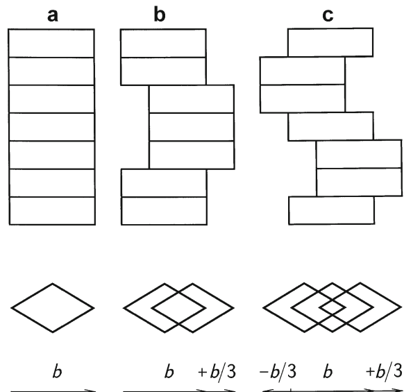
Figure 1. (a) Domains of cronstedtite-1T with origins at y = 0 only, (b) domains with origins at y = 0 and y = +\mathbf{b}/3 , (c) domains with origins at y = 0 , y = +\mathbf{b}/3 and y = -\mathbf{b}/3 . Schematic yz (top) and xy (bottom) projections.
