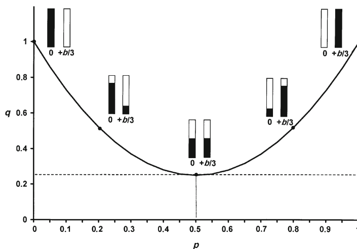
Figure 3. Plot of the function q = 3p^2 - 3p + 1 . The bar graphs correspond to some selected distributions of the basic structure between the positions with origins at y = 0 and y = +1/3 .
