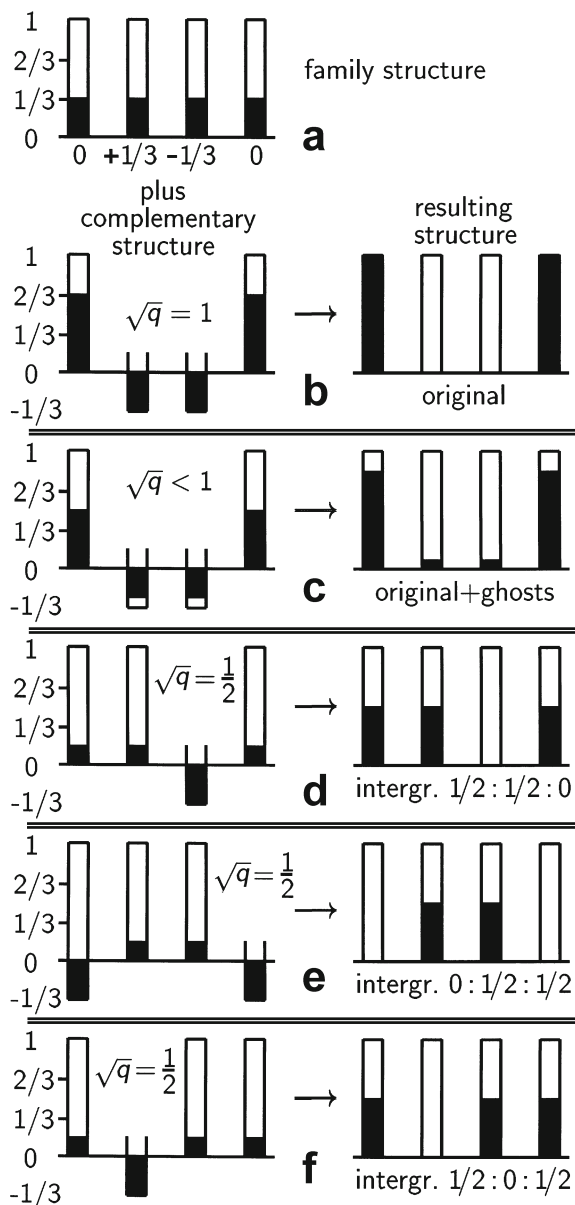
Figure 5. An illustration of how a single peak in a Fourier map at y=0 represented by a full column with unit height, appears in the Fourier map of the family structure (a) and in the Fourier maps of some selected complementary and resulting structures (b–f). Partly filled columns represent reduced peak heights in fractions of 1 as indicated along the vertical axis. Entries on the horizontal axis give fractional y coordinates 0, +1/3 and -1/3 = 2/3 as indicated in (a). (b) \sqrt{q} = 1 : resulting structure is the original one, (c) 1/2 < \sqrt{q} < 1 : phases of the complementary structure correspond to the original structure with origin at y=0 . (d–f) \sqrt{q} = 1/2 : phases of the complementary structures correspond to double intergrowths 1/2:1/2:0 (d), 0:1/2:1/2 (e) and 1/2:0:1/2 (f). Entries in the symbols for double intergrowths refer to the positions y = 0 , y = +1/3 and y = -1/3 , respectively.
