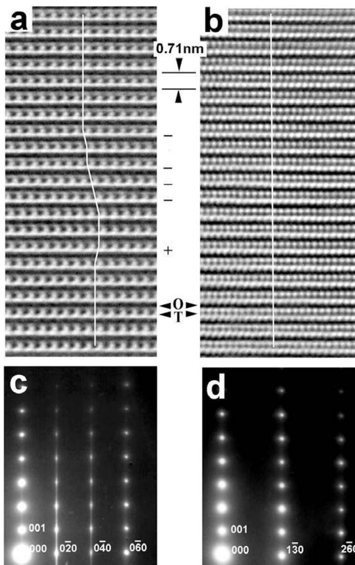
Figure 2. HRTEM images and SAED patterns from partially disordered 1 T -cronstedtite. The specimen is the apical part of a pyramidal crystal from Lostwithiel, England (Kogure et al. , 2002). Orthogonal indexing is used throughout. (a) HRTEM image along [100]. (b) HRTEM image along [310] recorded in almost the same area as in (a) but the specimen was rotated by 30° in the TEM. (c) SAED pattern along [100] from the same area as in (a). (d) SAED pattern along [310] from the same area as in (c). O and T indicate the positions of octahedral and tetrahedral sheets, respectively, in a unit layer (see Kogure et al. , 2001 for interpretation of the HRTEM images). The white line connecting equivalent positions in each layer, shows the lateral stagger between adjacent layers at the interlayer positions indicated with '+' or '-' in (a) whereas there is no stagger in (b). Streaks that are a consequence of stacking disorder are apparent along 0kl ( k \neq 3n ) reciprocal lattice rows in (c) whereas no streaks are observed in (d). All images and patterns were recorded using a JEOL JEM-2010 operated at 200 kV. The point resolution is ~0.2 nm
