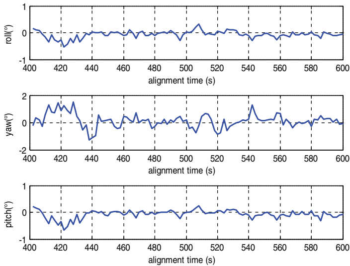
Figure 8. Roll errors (top), Yaw errors (middle), and pitch errors (bottom) over 400 seconds
