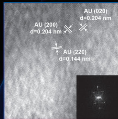
1.4Å Au (220) lattice at 100kV
