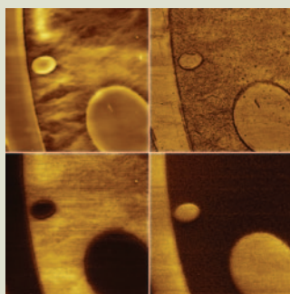
AFM images of a polymer blend. Lower squares show IR images characteristic of each component polymer. Image width = 20 \mu\text{m} .
