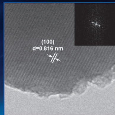
8.1Å (100) Hydroxyapatite lattice at 40kV
