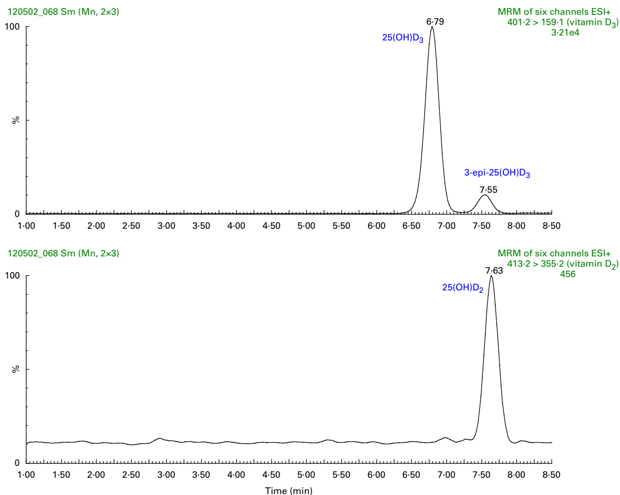
Fig. 1. Liquid chromatography–positive-ion electrospray ionisation (ESI) tandem MS chromatograms of 25-hydroxyvitamin D 3 (25(OH)D 3 ), 3-epimer of 25(OH)D 3 (3-epi-25(OH)D 3 ) and 25(OH)D 2 in a serum sample. MRM, multiple reaction monitoring. A colour version of this figure can be found online at http://www.journals.cambridge.org/bjn
