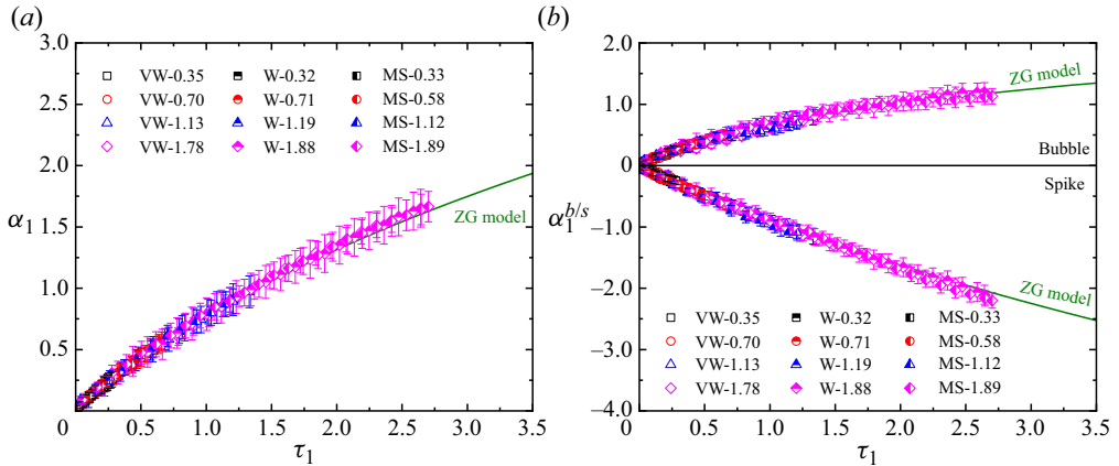
Figure 6. Experimental and theoretical results of the amplitude evolutions of the once-shocked interface (a) and its bubble and spike (b).
