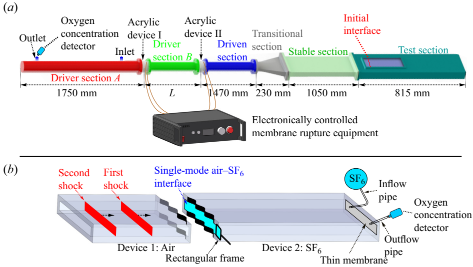
Figure 1. Sketches of the shock-tube facility for generating two successive shocks (a) and the interface formation devices (b).
