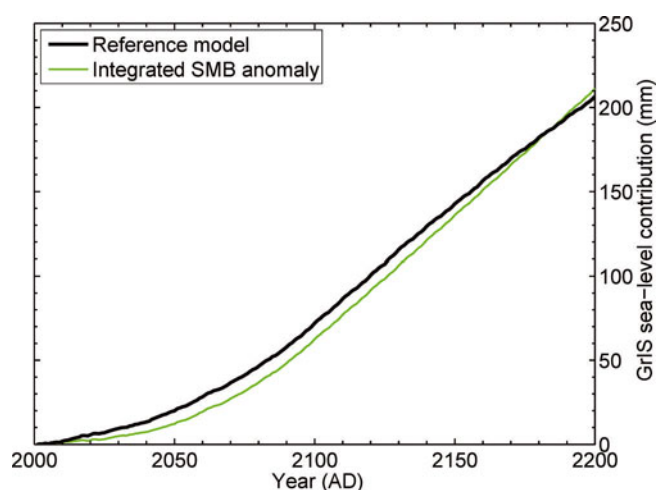
Fig. 6. Sea-level contributions projected with the reference model including ice dynamics and prescribed outlet glacier retreat compared to the time-integrated SMB anomaly as a measure of the direct SMB effect.
