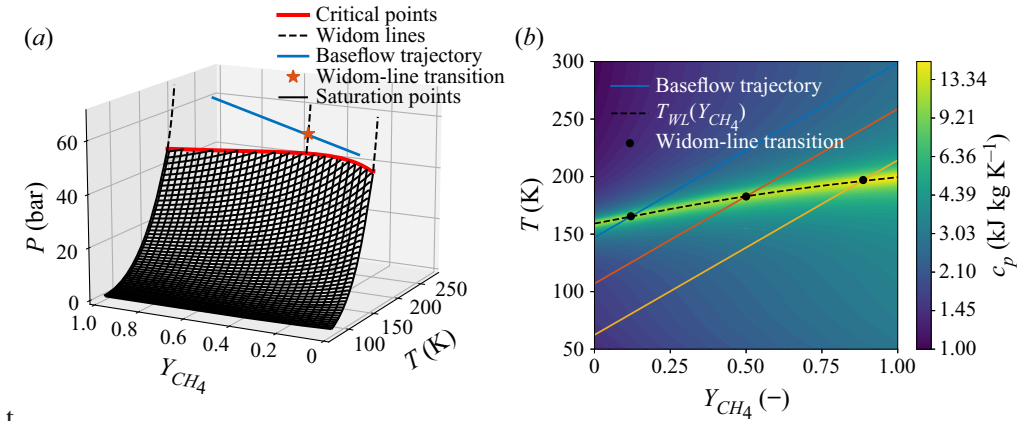
Figure 1. (a) Thermodynamic regime diagram of CH 4 /O 2 mixture at subcritical and supercritical conditions. Also plotted is the locus of thermodynamic conditions found in a representative isobaric baseflow. (b) Isobaric state space: isobaric projection of the supercritical thermodynamic regime diagram of CH 4 /O 2 at P = 60 bar, showing contour of isobaric heat capacity ( c_p ). Also shown is the Widom-line transition temperature as a function of composition T_{WL}(Y_{CH_4}) and example isobaric thermodynamic trajectories of the baseflow.
