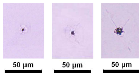
Figure 7. Morphology of the LID bulks in Figure 6.
